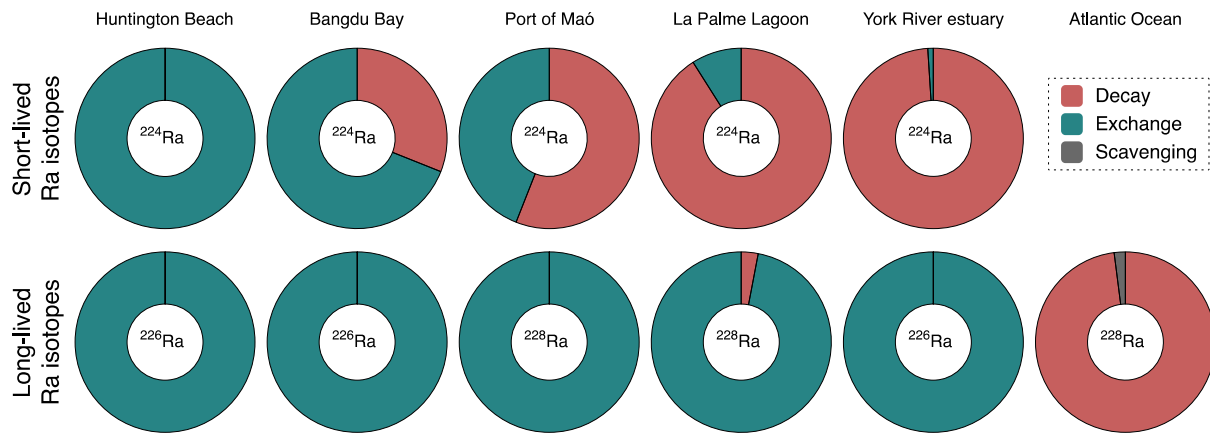
Fig. 9. Relative contribution of different sinks (decay, exchange and scavenging) to the total 224 Ra (upper row) and long-lived Ra isotopes (lower row) outputs for six study sites with distinct characteristics (see Fig. 8 for site references and details).
