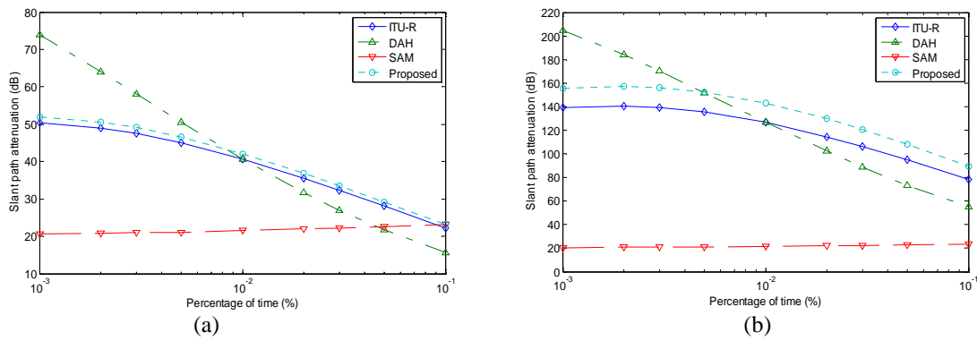
Fig. 8 Slant path exceedance for UTM at (a) 20 GHz, and (b) 40 GHz.
