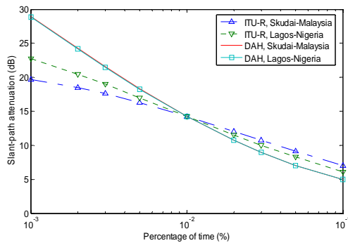
Fig.4 Slant-path Attenuation plot for Nigeria and for Malaysia at 12 GHz for 0.001% - 0.1% of the time in an average year.
