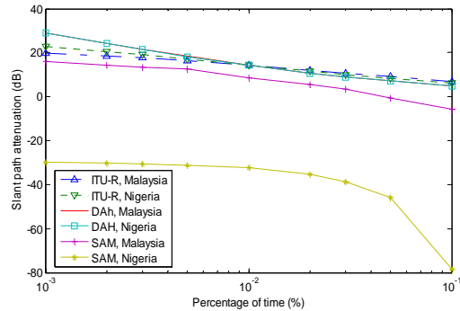
Fig.5 Comparison of slant-path attenuation plot at 12 GHz for UTM, Malaysia for 0.001- 0.1 % of the time in an average year.
