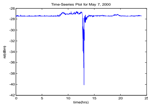
Figure 2. Time-Series plot for May7, 2000 at 38GHz for UTM, Malaysia
