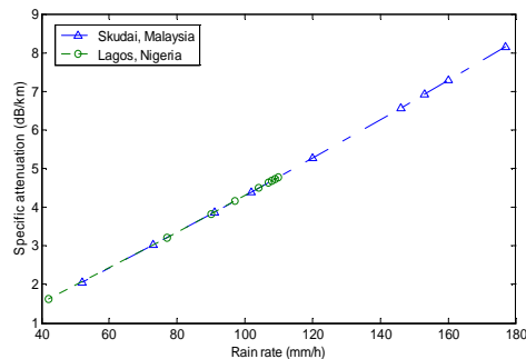
Figure 3. Comparison of plots of specific attenuation for Nigeria and Malaysia 12GHz in an average year.
