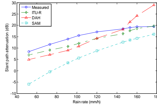
Fig. 7 Equal Probability plots of rain rate and slant path attenuation at 12 GHz for UTM, Malaysia.
