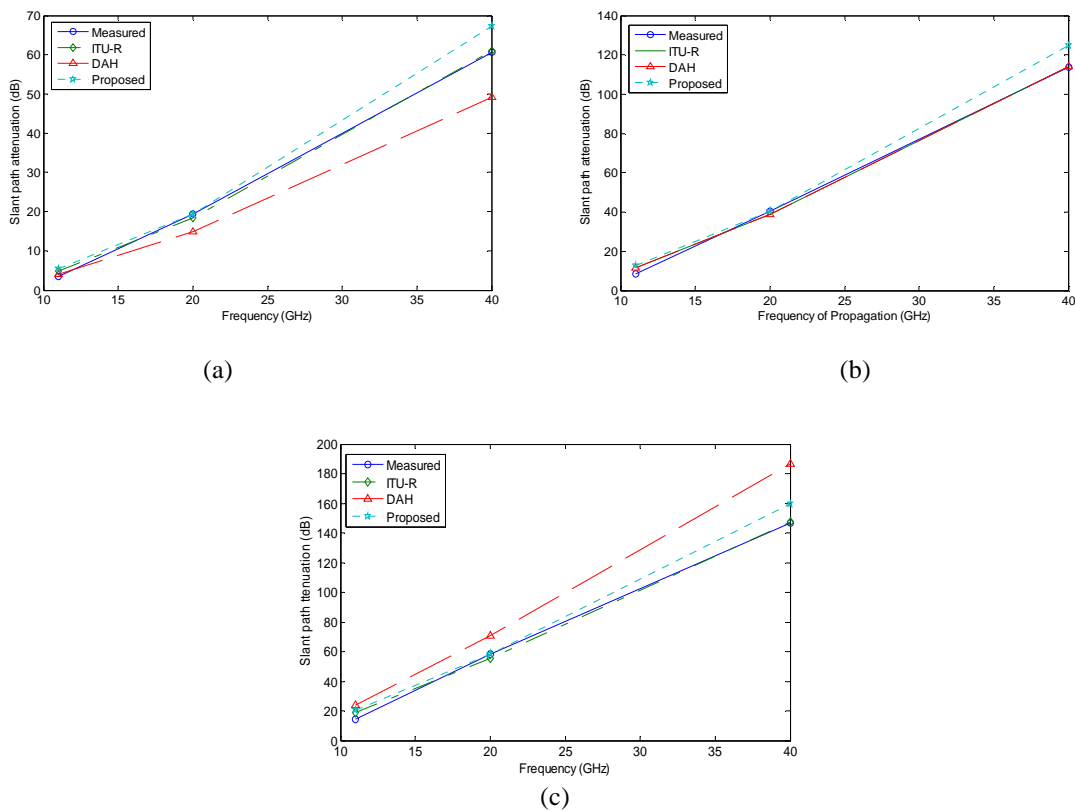
Fig. 9 Relationship between slant path attenuation and frequency for Lagos at (a) 0.1% (b) 0.01% and (c) 0.001% of time.
