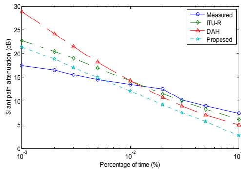
Fig. 6 Comparison of the Slant path attenuation exceedance at 12 GHz for Lagos, Nigeria.
