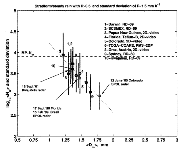
FIG. 10. The average value of \log_{10}\langle N_w \rangle (with \pm 1\sigma std dev bars) vs average D_m from disdrometer data and radar retrievals as indicated for stratiform rain. Dotted straight line is the least squares fit.
