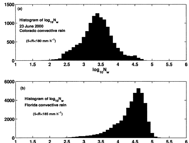
FIG. 7. As in Fig. 6, except histogram of \log_{10} N_w (units of N_w in \text{mm}^{-1} \text{m}^{-3} ).
