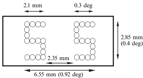
Figure 1. The LED display unit used as the foveal task for the experiment. Note that the characters are highly visible subtending 0.4 \text{ deg} \times 0.3 \text{ deg} . Sketch not to scale.
