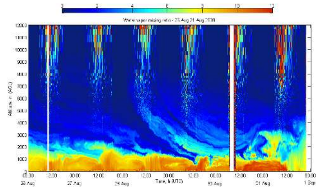
Fig. 14. Six-day time series of water vapor with 10 min time resolution. All data are shown, including data with a statistical error > 10\% . The noisy zones above 5000 m (around noon) mark the increase in statistical error due to the solar background during the daytime. The white zones mark data gaps.
