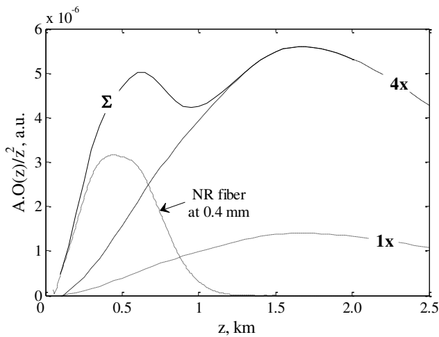
Fig. 6. Simulated signals in terms of AO(z)/z^2 disregarding the atmospheric transmission: signal from one telescope (1x), signal from four telescopes (4x), total signal from four telescopes including the contribution of the near range fiber ( \Sigma ).
