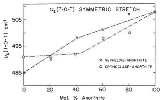
Fig. 5. \nu_s(T-O-T) as a function of composition in the spectra of glasses along the Or-An and Ne-An joins.
