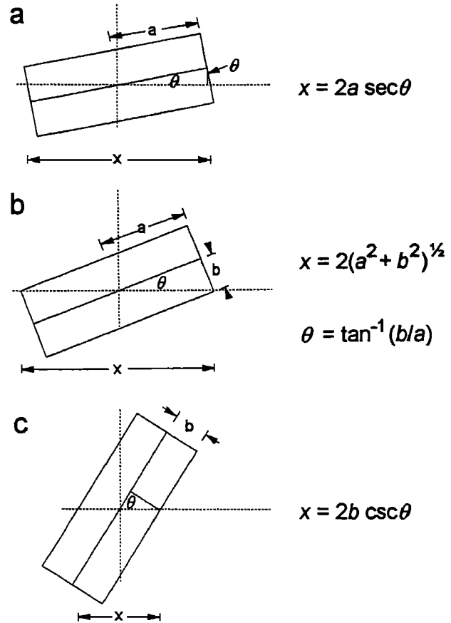
Figure A1. Schematic diagram of a rectangular grain and equations for determining the traverse distance along the X axis as a function of the angle \Theta between the X axis and the long axis of the crystal.
