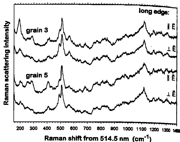
Figure 6. Spectra of two plagioclase grains in the thin section of 14161,7062, rotated from their long edges parallel to \bar{E} to perpendicular to \bar{E} . Note the change in spectral pattern and relative peak heights on rotation for each grain, and note the difference in spectral patterns between the two grains, which arises because of different grain orientations relative to the axis of the laser beam. As in Figure 5, spectra are offset from each other along the ordinate.
