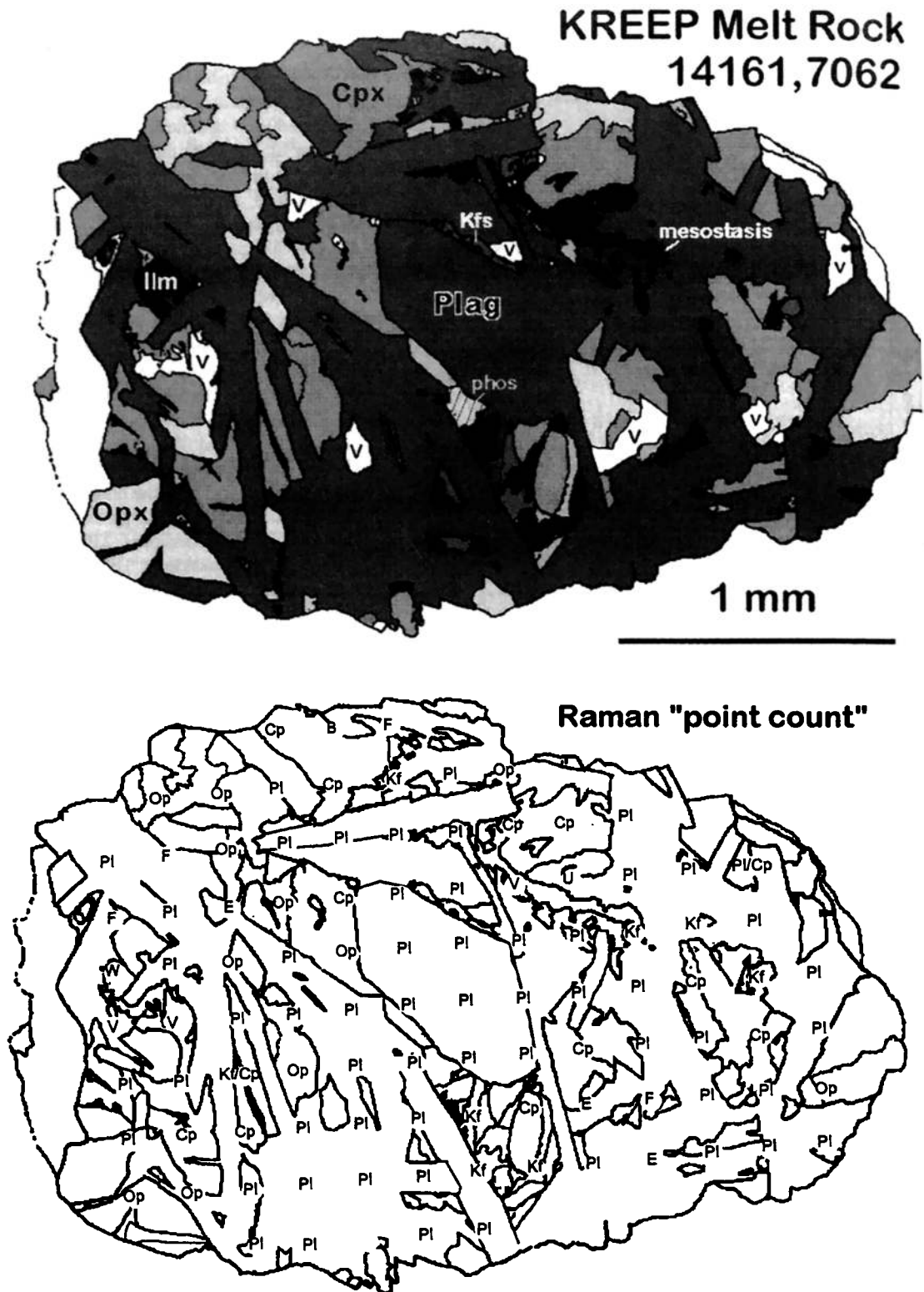
Figure 1. (a) Mineral map of thin section 14161,7062 KREEPy impact-melt rock fragment. Grain identifications and grain boundaries are based on reflected-light and backscattered-electron image (BEI) mosaics. The rock is rich in plagioclase and has a coarse, intergranular texture with pyroxene grains and areas of fine-grained mesostasis filling the spaces between the plagioclase mesh. In this map, the darkest mineral grains are mostly ilmenite (Ilm); slightly less dark are areas of undifferentiated mesostasis; plagioclase (Plag) is intermediate gray, K-feldspar (Kfs) is slightly lighter and occurs in areas of mesostasis, clinopyroxene (Cpx) and orthopyroxene (Opx) are lighter shades of gray and form large, composite pyroxene grains; and areas of voids (V) are white. (b) Grain boundary map of 14161,7062 showing locations and identifications of micro-Raman spot analyses. Pl, plagioclase; Cp, clinopyroxene, including pigeonite and augite; Op, orthopyroxene; Kf, K-feldspar; B, baddeleyite; W, whitlockite; E, epoxy; F, fluorescence; and V, void. The numbering scheme (see Table 1) begins with point 1 as the leftmost point in the top row, and numbering is sequential from upper left to lower right.
