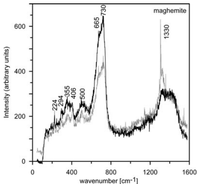
Figure 8. Raman spectra of maghemite produced by heating of lepidocrocite to 400\text{ }^{\circ}\text{C} . Again, some small haematite peaks are visible because part of the sample is oxidized. Grey line, 0.01\text{ mW} , 15\text{ min} ; black line, 0.1\text{ mW} , 3\text{ min} .
