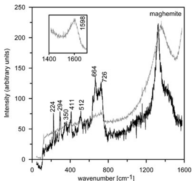
Figure 7. Raman spectra of maghemite produced by heating of natural ferrihydrite to 700\text{ }^{\circ}\text{C} . One of the spectra (black, 0.01\text{ mW} , 5\text{ min} ) shows small hematite peaks. The bands at 350 , 512 , 664 , 726 and 1330\text{ cm}^{-1} are attributed to maghemite. The grey spectrum ( 0.01\text{ mW} , 20\text{ min} ) was obtained at a different spot in the sample. Here, no haematite is present. The band above 1300\text{ cm}^{-1} is broader than for the black spectrum and an additional band exists at about 1600\text{ cm}^{-1} . This might point to the presence of burnt organic matter.
