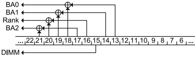
Fig. 1: Reverse engineered DDR3 single channel mapping (2 DIMM per channel) for Ivy Bridge / Haswell (from [49]).
