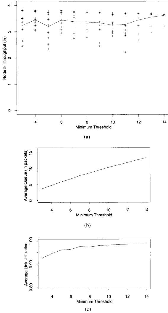
Fig. 14. Simulations with RED gateways
