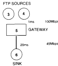
Fig. 6. Simulation network.
