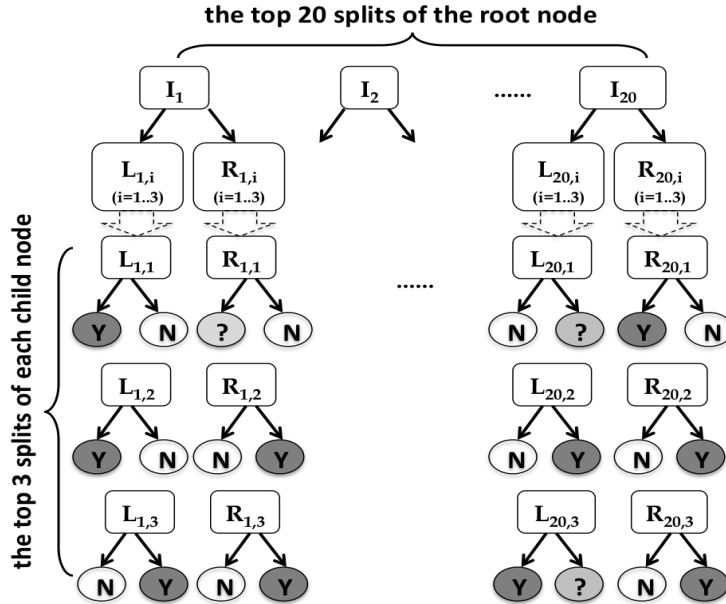
Fig. 1 A schematic illustration of the “deterministic forest” method for binary classification (proposed in [48]). I_1, \dots, I_{20} are the top 20 splits of the root node. Each of these top splits leads to a left ( L ) and a right ( R ) child node. The child nodes have their own splits ( L_{j,i} and R_{j,i} , where j \in \{1, \dots, 20\} and i \in \{1, 2, 3\} ). Three top splits are drawn underneath each of them. Based on the combinations of the root splits ( I_1, \dots, I_{20} ) and the child splits ( L_{j,i} and R_{j,i} ), the method made multiple trees with different terminal nodes (circles). The terminal nodes are color-coded based on the counts of two classes. The more positive examples a terminal node has, the more black it is. Nodes with “?” contain examples from both classes.
