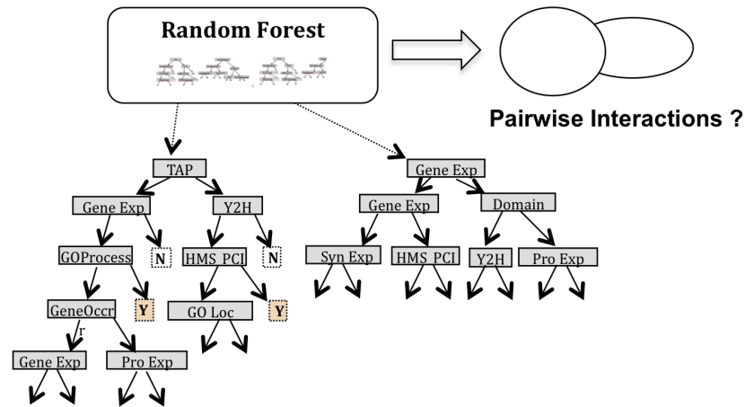
Fig. 5 Evidence was integrated using a random forest classifier for protein-protein interaction prediction. Figure modified from [35].
