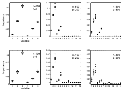
Figure: Variable importance sensitivity to n and p : second row ( n = 100 )
