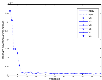
Figure: Variable selection procedure: Elimination
