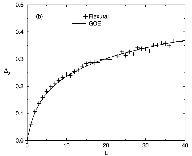
FIG. 10. The level spacing distribution (a) and the \Delta_3 statistic (b) for the flexural modes compared with the GOE statistics. Both the level spacing distribution and the \Delta_3 statistic agree very well with the GOE results.
