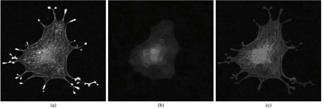
Fig. 5. Original ( \mathbf{I} ), marker ( \mathbf{M} ) and simplification by h -depth vector leveling \Lambda_{h_{\mathbf{T}}}(\mathbf{I}, \mathbf{M}) . The marker \mathbf{M} is the product of a h -depth closing followed by an h -depth opening with the SE is a disk of size 10. (a) \mathbf{I} ; (b) \mathbf{M} = \gamma_{SE, h_{\mathbf{T}}}(\phi_{SE, h_{\mathbf{T}}}(\mathbf{I})) ; (c) \Lambda_{h_{\mathbf{T}}}(\mathbf{I}, \mathbf{M}) .
