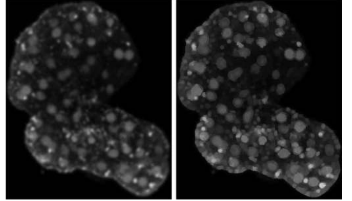
Fig. 4. Edge enhancement of \mathbf{I} using toggle mapping \tau_{h_{\mathbf{I}}}(\mathbf{I}) in the proposed ordering. Source: http://www.cellimagelibrary.org/
