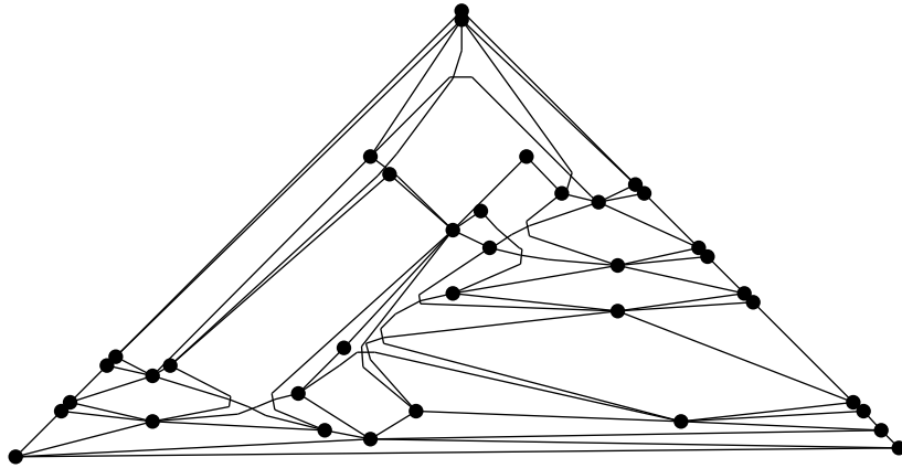
Figure 13: Intermediate result of Fig. 12 after the drawing algorithm.
