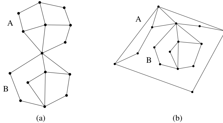
Figure 3: The unified face of two biconnected components, shown after removal of the dummy edge, and drawn as external (a), and interior (b).
