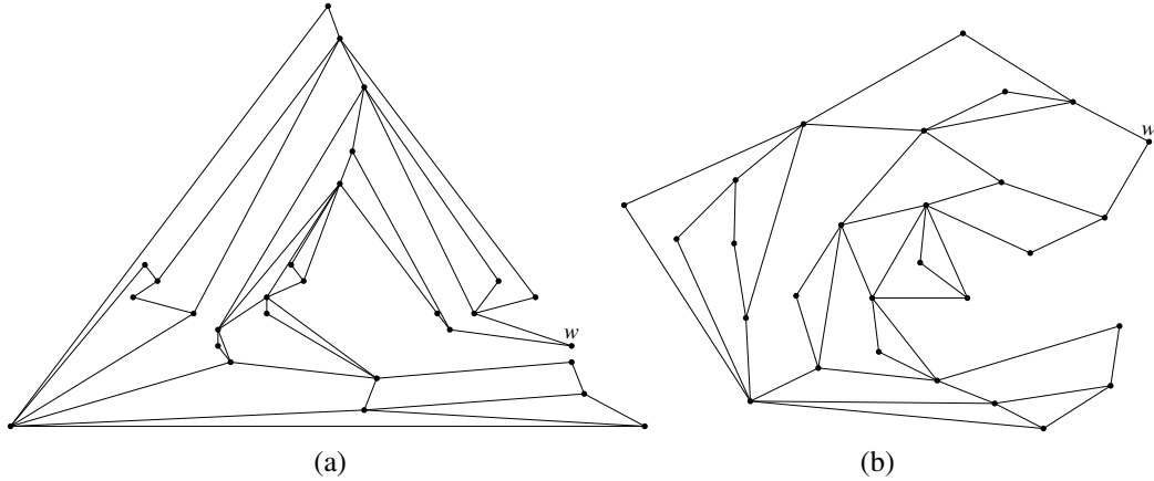
Figure 1: The problematics of naively applying the drawing algorithm to a non-triangulated graph.
