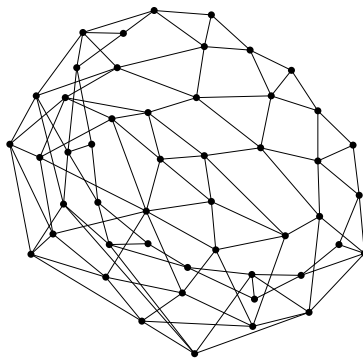
Figure 9: The graph of Fig. 7 as produced by the simulated annealing system of [DH89].
