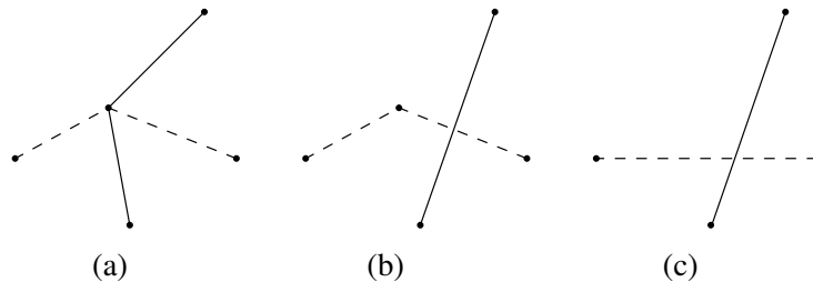
Figure 5: Straightening bends in two stages: (a) the dummy vertex, (b) after the first stage, (c) after the second stage.
