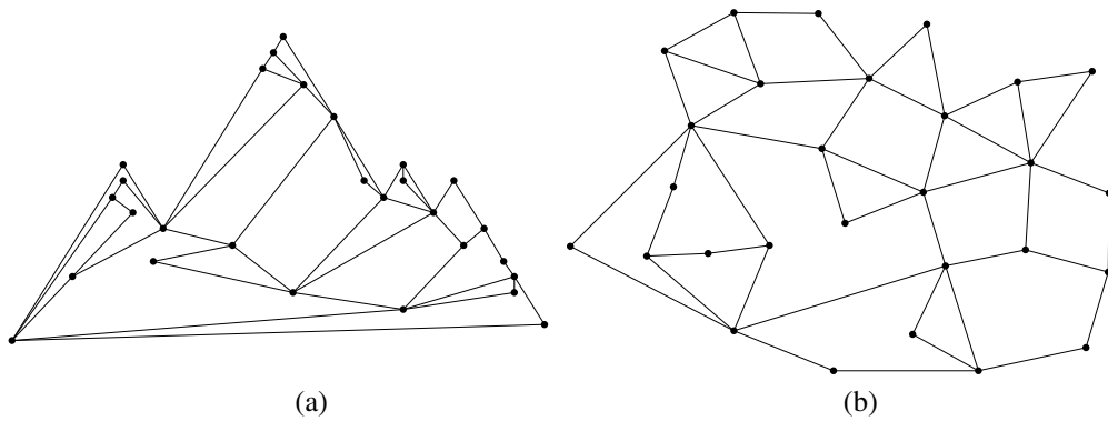
Figure 2: The graph from Fig. 1 as drawn by our system.
