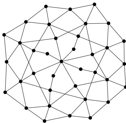
Figure 12: Final result on a non-planar graph of 37 vertices and 76 edges.
