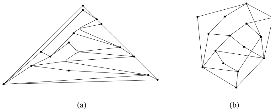
Figure 6: A graph drawn using the shortest face-path heuristic.
