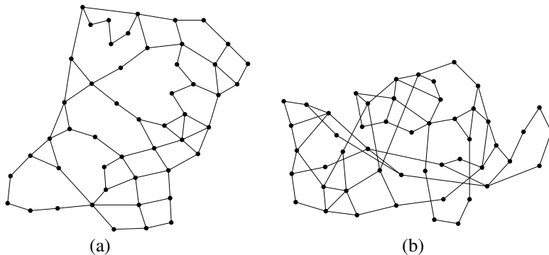
Figure 10: A sparse planar graph: (a) our system’s output, and (b) that of the annealing system of [DH89].
