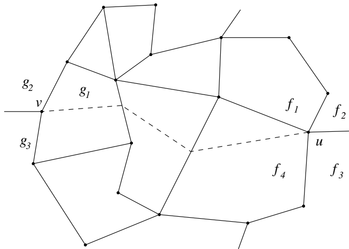
Figure 4: Adding a quasi-edge using the short face-path heuristic.
