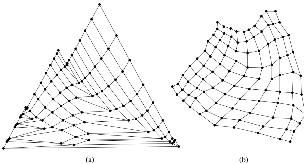
Figure 11: A 10-by-10 grid: (a) after planarization, (b) the system's final result
