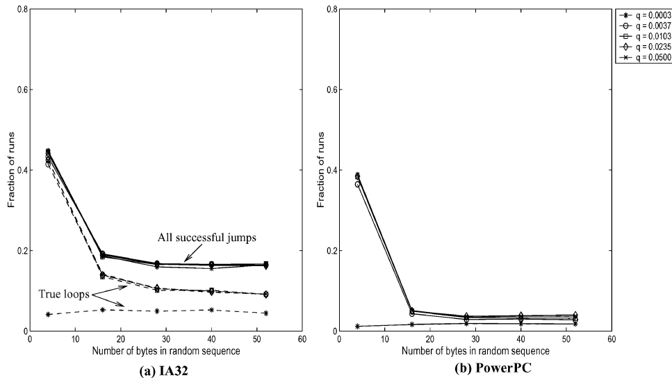
Fig. 3. Probability that random code escapes when executed for different block sizes (the x -axis) for (a) IA32 and (b) Power PC. Block size is the length of the sequence of random bytes inserted into the process. Each set of connected points represents a different memory density ( q ). Solid lines represent the fraction of runs that escaped under our definition of escape, and dotted lines show the fraction of “true” escaped executions (those that did not fail after escaping from the exploit area).
