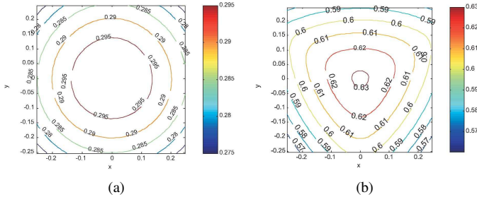
Fig. 11. Contour plots of (a) \kappa(J_z) and (b) \kappa(J_\Psi) at z = z_c and \eta = 0 .
