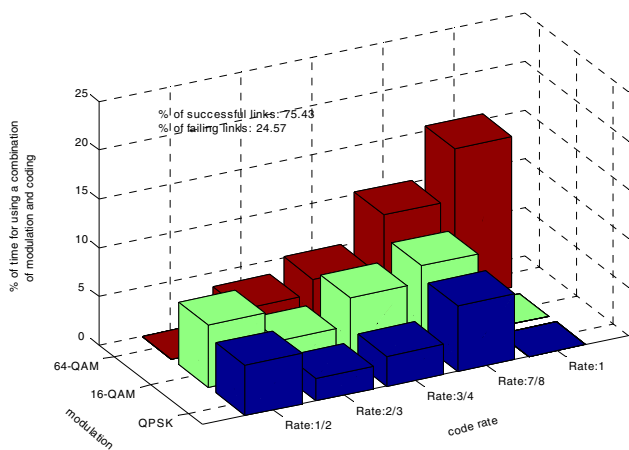
Fig. 6. 3-D histogram of adaptive modulation and coding usage (without relay, SINR-based relay selection algorithm, P_{relay} = 1 W, R = 1000 m).
