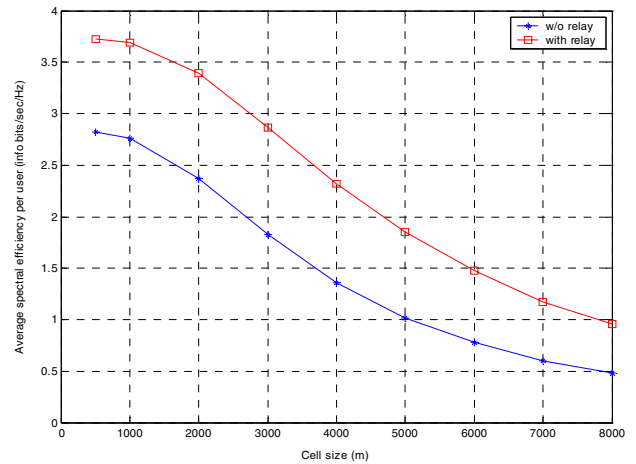
Fig. 3. Average spectral efficiency for various cell sizes (SINR-based relay selection algorithm, P_{relay} = 1 W).
