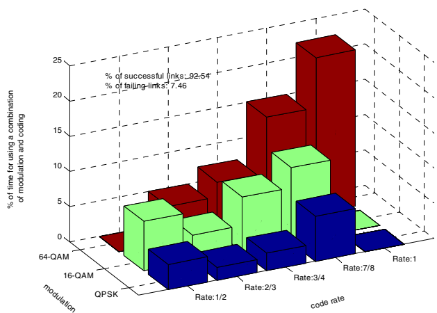
Fig. 7. 3-D histogram of adaptive modulation and coding usage (with relay, SINR-based relay selection algorithm, P_{relay} = 1 W, R = 1000 m).
