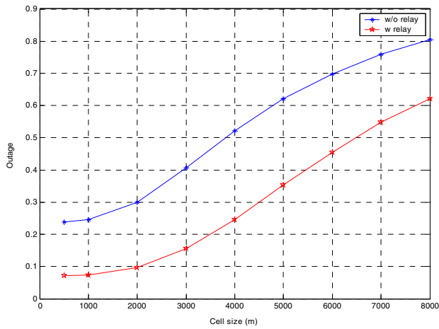
Fig. 4. Outage results for various cell sizes (SINR-based relay selection algorithm, P_{relay} = 1 W).
