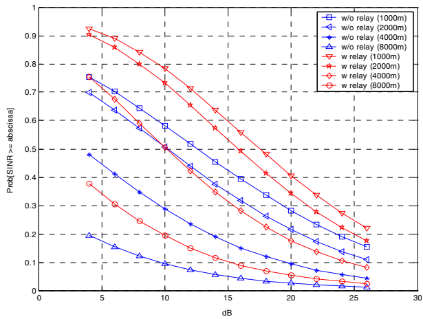
Fig. 2. Coverage at various SINR levels (SINR-based relay selection algorithm, P_{relay} = 1 W).
