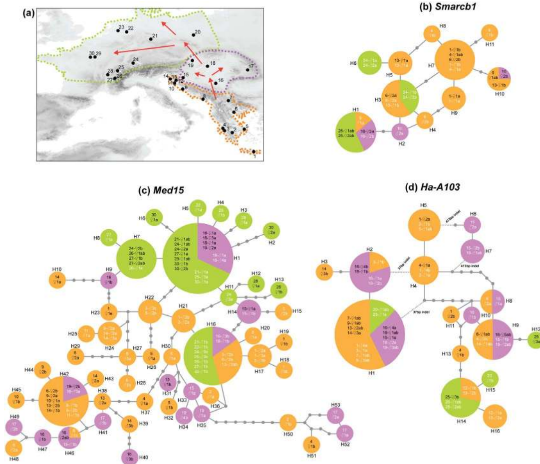
Figure 1. Sampling localities (a) and haplotype networks of Smarcb1 (b), Med15 (c) and Ha-A103 (d). For each allele, labels indicate locality number, followed by the sex of the individual (black for females and white for males), a sample number, and the letter a or b (discriminating two alleles of heterozygotes; written "ab" for homozygotes). The colors of haplotypes correspond to the main phylogeographic regions across H. arborea 's present distribution range (as described by Stöck et al. 2012, and Dufresnes et al. 2013), delimited by thin dashed lines on the map (orange: southeastern European refugia; violet: Pannonian basin; green: NW Europe). Arrows show post-glacial recolonization routes. doi:10.1371/journal.pone.0097959.g001
