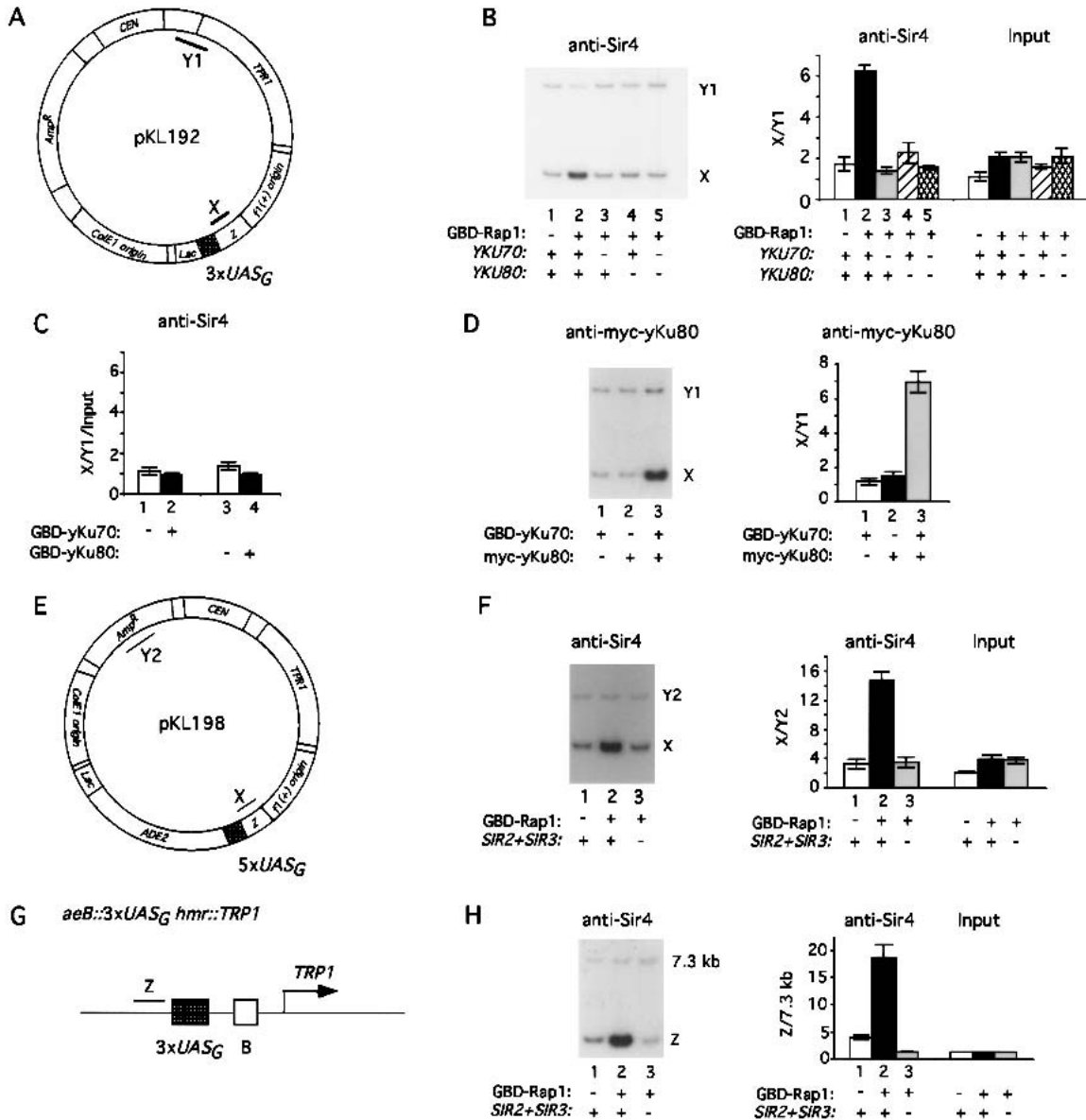
Figure 5. Sir4 recruitment by Rap1 depends on YKU70/YKU80 , SIR2 , and SIR3 at nontelomeric sites. (A–D) yKu70/yKu80 are required for Sir4 recruitment by GBD–Rap1 on a plasmid. Plasmid pKL192 carrying 3× UAS C sites (Gal4 DNA-binding sites) and PCR amplification products used for ChIP are shown schematically in A. PCR fragment X is immediately next to the UAS C sites. Fragment Y1, which is 1.4 kb away from the UAS C sites, served as a background control. (B) Sir4 recruitment by GBD–Rap1 is abolished in yku70Δ and yku80Δ mutants. ChIP was carried out as described in Figure 1. The GBD–Rap1 fusion construct was cotransformed with pKL192 into wild-type (WT; AJL275–2a–VIII–URA; lanes 1,2), yku70Δ (KLY16; lane 3), yku80Δ (KLY17; lane 4), and yku70Δ yku80Δ (KLY161; lane 5) strains. Sir4 association with pKL192 was analyzed. The ratio of enrichments at X versus at Y1 was plotted. (C) GBD– yKu70 and GBD– yKu80 do not recruit Sir4 to pKL192. GBD alone (lane 1,3), GBD– yKu70 (lane 2), and GBD– yKu80 (lane 4) constructs were cotransformed with pKL198 into wild-type (WT; AJL275–2a–VIII–URA), respectively. Sir4 association with pKL192 was analyzed as in B. The ratio of enrichments at X versus at Y1 was plotted after normalization with Input DNA. (D) yKu70 and yKu80 interact at pKL192. GBD– yKu70 was transformed with pKL192 into a strain carrying a myc -tagged yKu80 (GA1009). Antibody specific to the myc tag was used to examine myc - yKu80 binding on pKL192 in strains carrying wild-type yKu80 (GA426) and GBD– yKu70 (lane 1); myc - yKu80 (GA1009) and GBD alone (lane 2); and myc - yKu80 (GA1009) and GBD– yKu70 (lane 3). (E,F) Sir2 and Sir3 are required for Sir4 recruitment by GBD–Rap1 to plasmid pKL198. Plasmid pKL198 carrying 5× UAS C sites is shown schematically in E with regions amplified by PCR. PCR fragment X is immediately next to the UAS C sites. Fragment Y2 is 2.75 kb away from the UAS C sites and served as a background control. GBD (lanes 1) and GBD–Rap1 fusion (lanes 2,3) plasmids were cotransformed with pKL198 into wild-type (WT; RS1001; lanes 1,2) and sir2Δ sir3Δ (KLY111; lane 3) strains. Sir4 binding on pKL198 was analyzed as shown in F. The ratio of enrichments at X versus Y2 is plotted. (G,H) Sir2 and Sir3 are required for Sir4 recruitment by GBD–Rap1 to the HMR locus. The mutated hmr region is shown schematically in G (Chien et al. 1993). PCR fragment Z is immediately next to the 3× UAS C sites. The subtelomeric region at 7.3 kb from the right end of Chromosome VI served as a background control. GBD (lane 1) and GBD–Rap1 fusion (lanes 2,3) plasmids were transformed into wild-type (WT; RS1001; lanes 1,2) and sir2Δ sir3Δ (KLY111; lane 3) strains. Sir4 binding analyzed by ChIP is shown in H. The ratio of enrichments at Z versus 7.3 kb is plotted.
