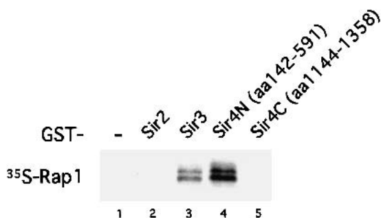
Figure 4. Rap1 binds Sir4 in vitro. In vitro binding of Rap1 and GST–Sir fusion proteins. GST–fusion protein experiments were performed as described in Materials and Methods. Full-length Rap1 was labeled in vitro with 35 S-Methionine and incubated with GST (lane 1), GST–Sir2 (amino acids 275–562, lane 2), GST–Sir3 (amino acids 503–970, lane 3), GST–Sir4N (amino acids 142–591, lane 4), and GST–Sir4C (amino acids 1144–1358, lane 5). Interacting proteins were analyzed by SDS-PAGE and fluorography.
