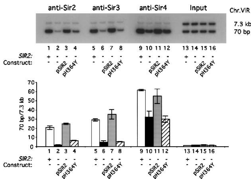
Figure 2. The deacetylase activity of Sir2 is required for Sir2 and Sir3, but not Sir4, to bind to the region 70 bp from the telomeric end. Sir protein binding to the region starting at 70 bp from the C_{1-3}A repeats was assayed in the wild-type (WT) strain (Y1195; lanes 1,5,9,13); the sir2 \Delta strain containing vector pRS315 (Y1201; lanes 2,6,10,14); the sir2 \Delta strain containing pSIR2 (Y1203; lanes 3,7,11,15), and the sir2 \Delta strain containing pH364Y (Y1205; lanes 4,8,12,16). ChIP and PhosphorImager quantitations were performed as described in Figure 1 and are shown as fold enrichment at 70 bp compared with that at 7.3 kb.
