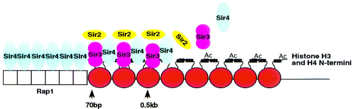
Figure 6. Model for the initiation and spreading of telomeric heterochromatin. Sir4 is the first Sir protein recruited to the telomere end by Rap1 to initiate the formation of the silencing complex. Sir4 recruits Sir2 and Sir3. Sir2 deacetylates histone tails to allow Sir3 binding to nucleosome(s) adjacent to the Rap1 sites. Sir3 recruits more Sir4 onto nucleosomes. The process is repeated as Sir4 recruits Sir2 and Sir3 and the complex propagates along the chromosome. The complex that initiates heterochromatin (detected at 70 bp from the telomeric end) differs from that which spreads (detected at 0.5 kb and beyond) in telomeric heterochromatin.
