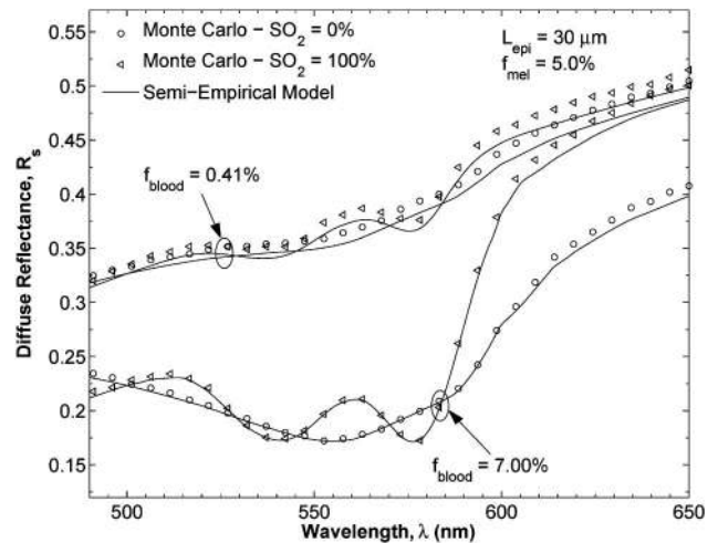
Fig. 3. Diffuse reflectance of human skin as a function of wavelength calculated by Monte Carlo simulations and predicted by the semiempirical model for L_{epi} = 30 \mu\text{m} and f_{mel} = 5.0\% and different values of blood volume fraction f_{blood} (0.41% and 7%) and oxygen saturation SO_2 (0 and 100%).
