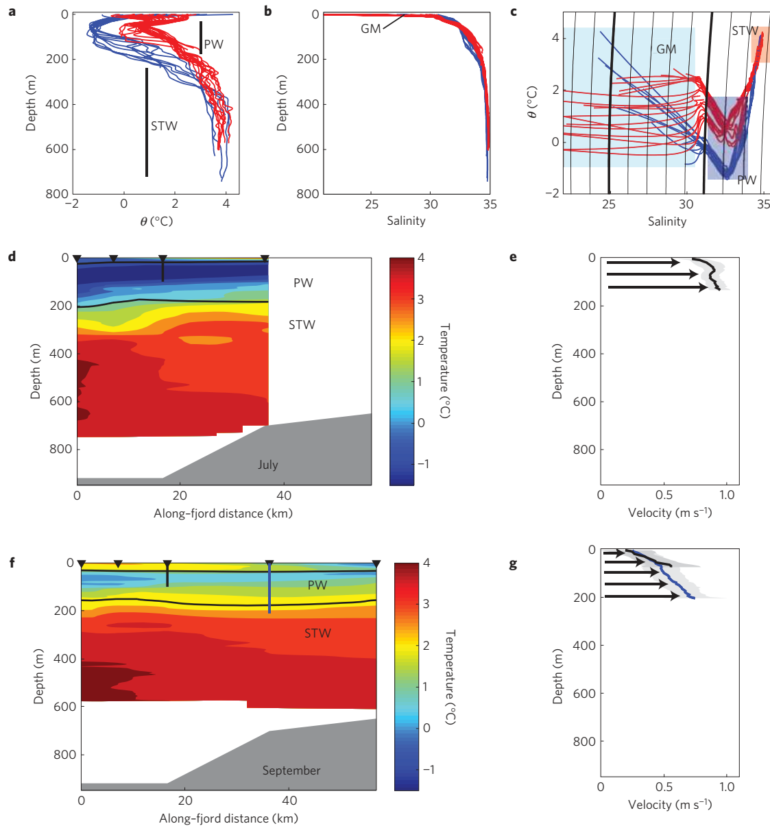
Figure 2 | Measurements in Sermilik Fjord in summer 2008 and the three water masses, GM, PW and STW. a , Potential temperature in July (blue) and September (red). b , Salinity (colours as a ). c , Potential temperature versus salinity (colours as a ). Potential-density contours are overlaid in black (thick lines are \sigma_\theta = 20 and 25 \text{ kg m}^{-3} ). d,f , Potential-temperature distribution in the along-fjord direction ( x = 0 is the mouth) from across-section averages, in July and September, respectively. The 31.5 and 34 isohalines are overlaid to separate the three layers. Top triangles indicate section location and vertical bars the velocity sections. Bathymetry is shaded in grey. e,g , Along-fjord velocity averaged across fjord at the sections indicated in d and f , respectively; positive is towards the head of the fjord. Shading indicates the standard deviation across the section; arrows indicate the direction of flow.
