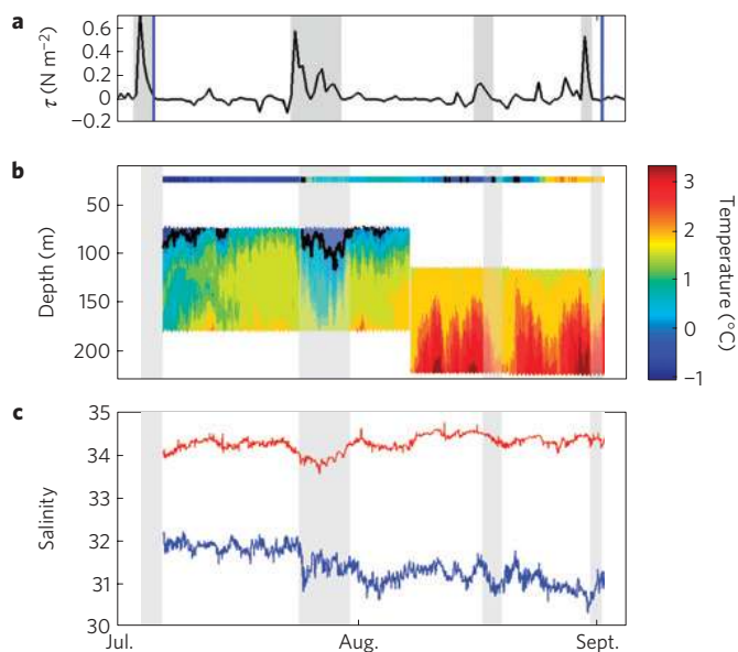
Figure 4 | Along-shore winds in Sermilik Fjord. a , Northeasterly wind stress outside Sermilik Fjord from Quikscat. Wind events are shaded (see Supplementary Methods). Blue lines show when the velocity data were collected. b , Potential temperature from the two summer moorings. Data from the 11 temperature recorders were vertically interpolated. The deep mooring was hit by ice and relocated 40 m deeper in early August. Wind events are as in a but lagged by one day (see Supplementary Methods). c , Salinity from the two moorings at 25 m (blue) and at 180–200 m (red). Shaded regions are as in b .
