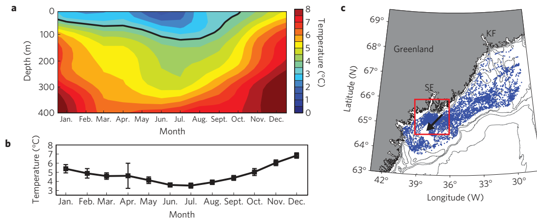
Figure 3 | Seasonal temperature variation on the East Greenland Shelf from tagged hooded seals. a , Monthly and spatially averaged temperature profiles versus depth (the solid line is 3.5 °C and approximately separates the PW from the STW). b , Mean monthly temperature averaged over the upper 400 m (vertical bars indicate standard error). c , Locations of the 5,269 seal dives. Both the winds and the heat fluxes referred to in the text were averaged over the red box shown. The direction of the northeasterly winds (oriented at 54°) is shown by the black arrow.
