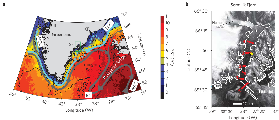
Figure 1 | Circulation around southeast Greenland and Sermilik Fjord. a , Currents around Greenland overlaid on the 2003 mean sea-surface temperature from the Advanced Very High Resolution Radiometer (filled contours). Bathymetric contours (100, 500, 1,000, 2,000, 3,000 m) are overlaid in black. PW transported by the EGC and WGC is in blue (dashed paths indicate multiple branches) and STW transported by the NAC and IC in grey. Sermilik Fjord (SF, green box), Kangerdlugssuaq Fjord (KF) and Jakobshavn Isbrae (JI) are indicated. b , Landsat mosaic of Sermilik Fjord. Sections (1–4, S) plus station A occupied in the 2008 surveys are indicated in red, moorings' locations by the yellow star.
