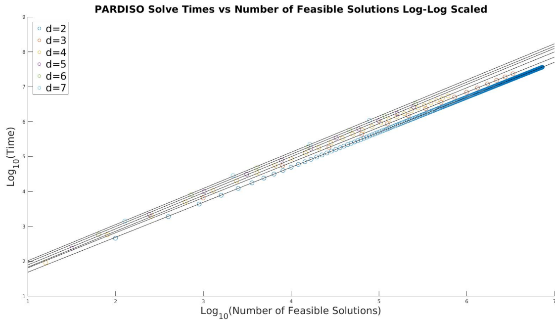
Figure 3 Log-log plot of times to solve a single-column right-hand-side vector system with \bar{Q} for problems of different dimension, d , and number of feasible solutions, n .
