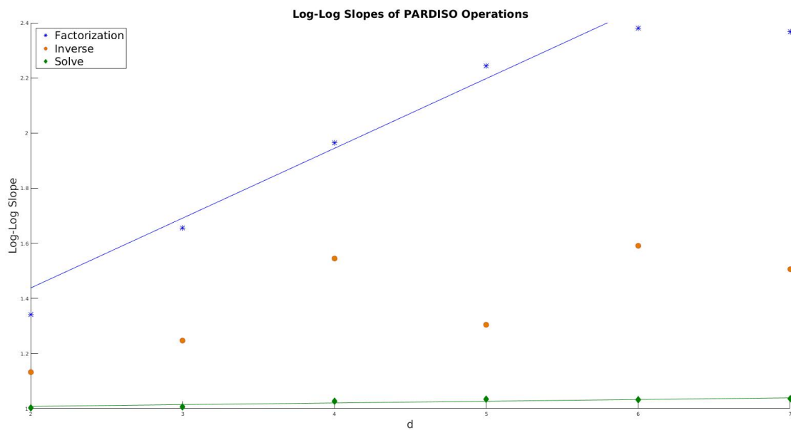
Figure 4 Slopes of log-log linear regression of PARDISO operations times vs. number of feasible solutions as a function of dimension, d .
