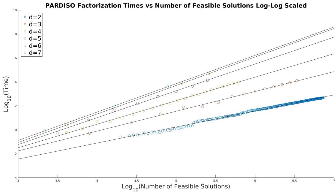
Figure 1 Log-log plot of times to compute Cholesky factorizations of \bar{Q} for problems of different dimension, d , and number of feasible solutions, n .
