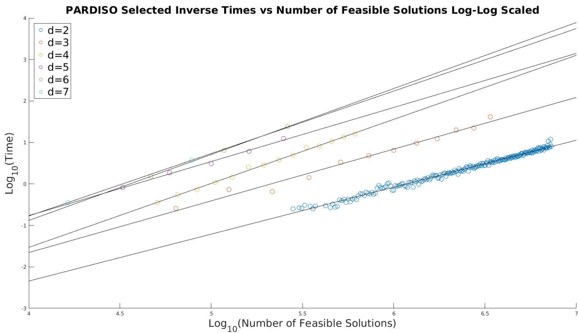
Figure 2 Log-log plot of times to compute selected inverse of \bar{Q} for problems of different dimension, d , and number of feasible solutions, n .
