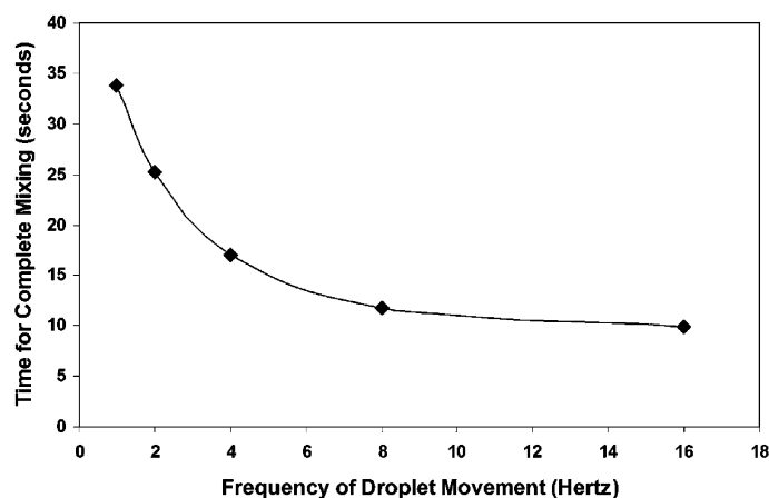
Fig. 6 Active mixing times as a function of switching frequency on a 2 × 2 electrode array. Note: the solid line is included for visualization purposes and is not meant to represent any curve fit.
