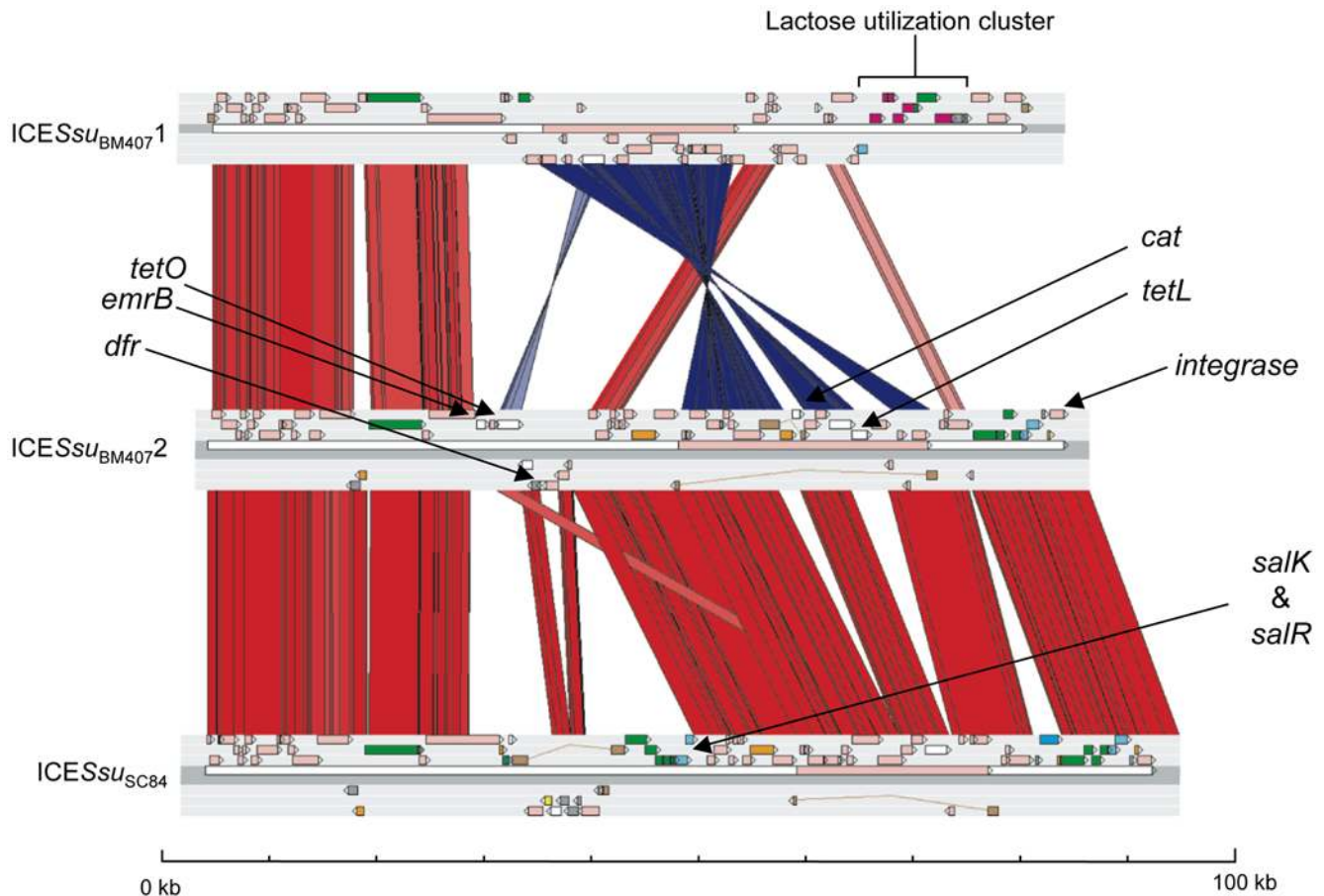
Figure 6. Comparisons of the ICE regions from S. suis strains BM407 and SC84. The results of a TBLASTX comparison of the ICES suBM4071 and ICES suBM4072 regions from strain BM407, and ICES suSC84 from strain SC84 is displayed using the Artemis Comparison Tool (ACT) [26]. doi:10.1371/journal.pone.0006072.g006
