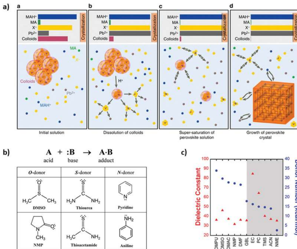
Fig. 6 (a) Schematic of the mechanism for crystallization of perovskite solid phase, where it represents the state of the system at several key points (reproduced with permission from ref. 124, ©2016 Springer Nature). (b) Representation of the Lewis acid (A)–base (B) reaction to form an adduct (A·B) with a dative bond and Lewis bases with different molecule donors (reproduced with permission from ref. 126, ©2016 American Chemical Society). (c) Dielectric constant (red triangles) and Gutmann's donor number ( D_N , blue circles) of solvents used for perovskite processing (reproduced with permission from ref. 127, ©2017 American Chemical Society).
