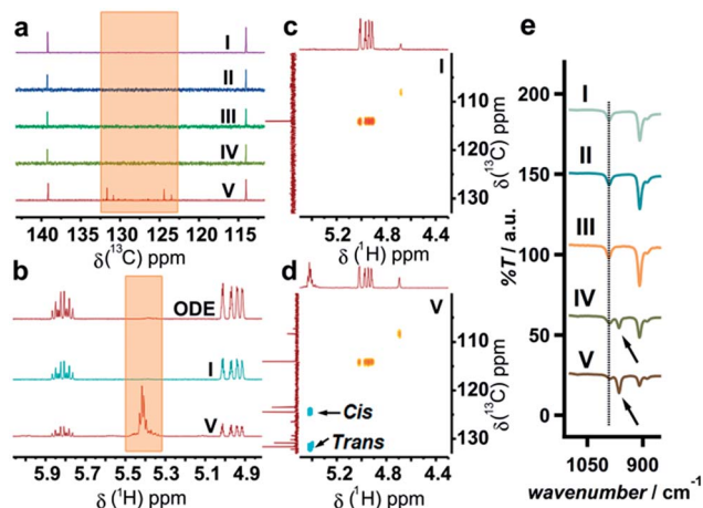
Fig. 1 13 C-NMR analysis of Se in 1-ODE at room temperature (step I), 60 °C for 30 min under vacuum (step II), 130 °C for 30 min under vacuum (step III), 200 °C for 30 min (step IV) and 20 h (step V) under Ar (a). 1 H-NMR spectra of the solution precursor at steps I and V, as well as of 1-ODE after heating at 200 °C for 20 h under Ar in the absence of Se (b). The highlighted areas in (a) and (b) correspond to the signal associated with the olefin functional group. HSQC 2D NMR spectra of Se containing solutions at step I (c) and step V (d). The arrows indicate the correlation between 13 C– 1 H from cis and trans olefin moieties. FTIR analysis of the precursor solutions at steps I to V (e). The arrows indicate a vibrational mode associated with the olefin moiety in trans 2-octadecene, while the dotted line indicates the position of the equivalent vibrational model in 1-ODE.
