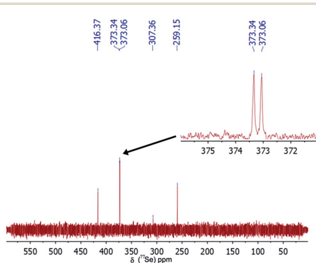
Fig. 2 Proton decoupled 77 Se NMR spectrum of the purified Se intermediate generated after dissolution of 1-ODE after 20 h at 200 °C under Ar. The inset shows two closed peaks with chemical shifts of 373.3 and 373.1 ppm.
