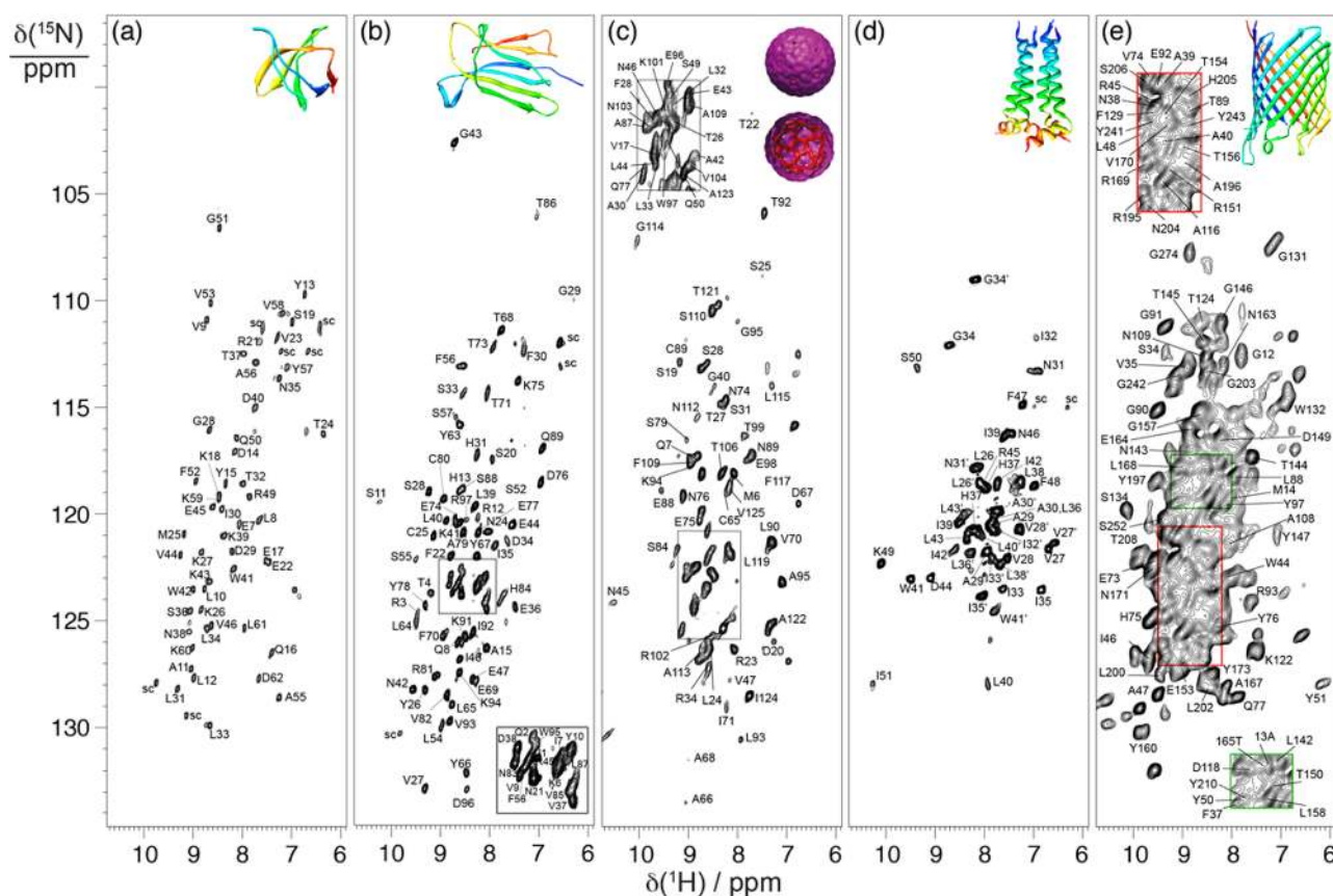
Figure 2. ^{15}\text{N} – ^1\text{H} correlation spectra recorded on a 1 GHz spectrometer under 60 kHz MAS for [\text{U}\text{-H}^{\text{N}}, ^2\text{H}, ^{13}\text{C}, ^{15}\text{N}] -labeled (a) microcrystalline SH3, (b) microcrystalline \beta 2\text{m} , and (c) sedimented nucleocapsids of AP205, (d) M2 channel, and (e) OmpG.
