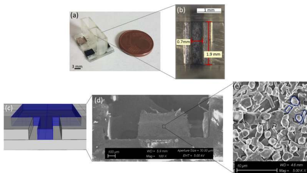
Figure 3. 3D printed OEECT. (a) Device after printing; (b) microscope image of the 700 \mu\text{m} wide channel; (c) section view of the 700 \mu\text{m} wide channel geometry; (d) FESEM image of the same section view reported in (c); (e) FESEM image of the PEGDA:PEDOT polymerized resin in which the PEDOT particles (some are highlighted in blue) are clearly visible.
