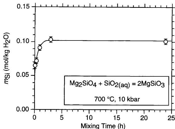
Fig. 5. Variation in the apparent solubility with the time of fluid mixing in an extraction vessel. Uncertainties are 2 sd ( \pm 0.008 mol/kg \text{H}_2\text{O} ).
