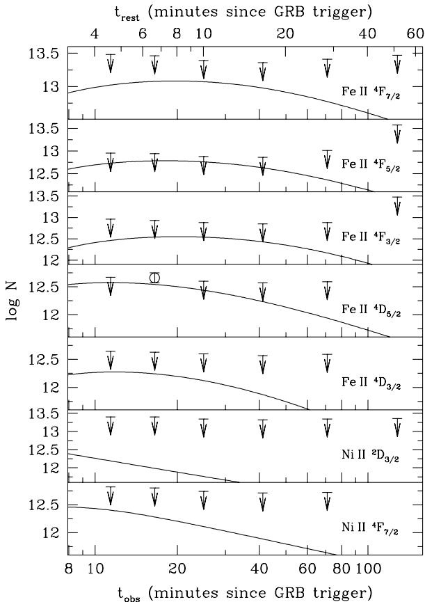
Fig. 9. Comparison of the UV-model predicted column densities for several additional Fe II and Ni II excited levels, i.e. others than the ones shown in Fig. 8, with the 5\sigma upper limits that we obtain from the spectra. The Fe II 4D_{5/2} level is actually detected at just above 5\sigma in the second epoch.
