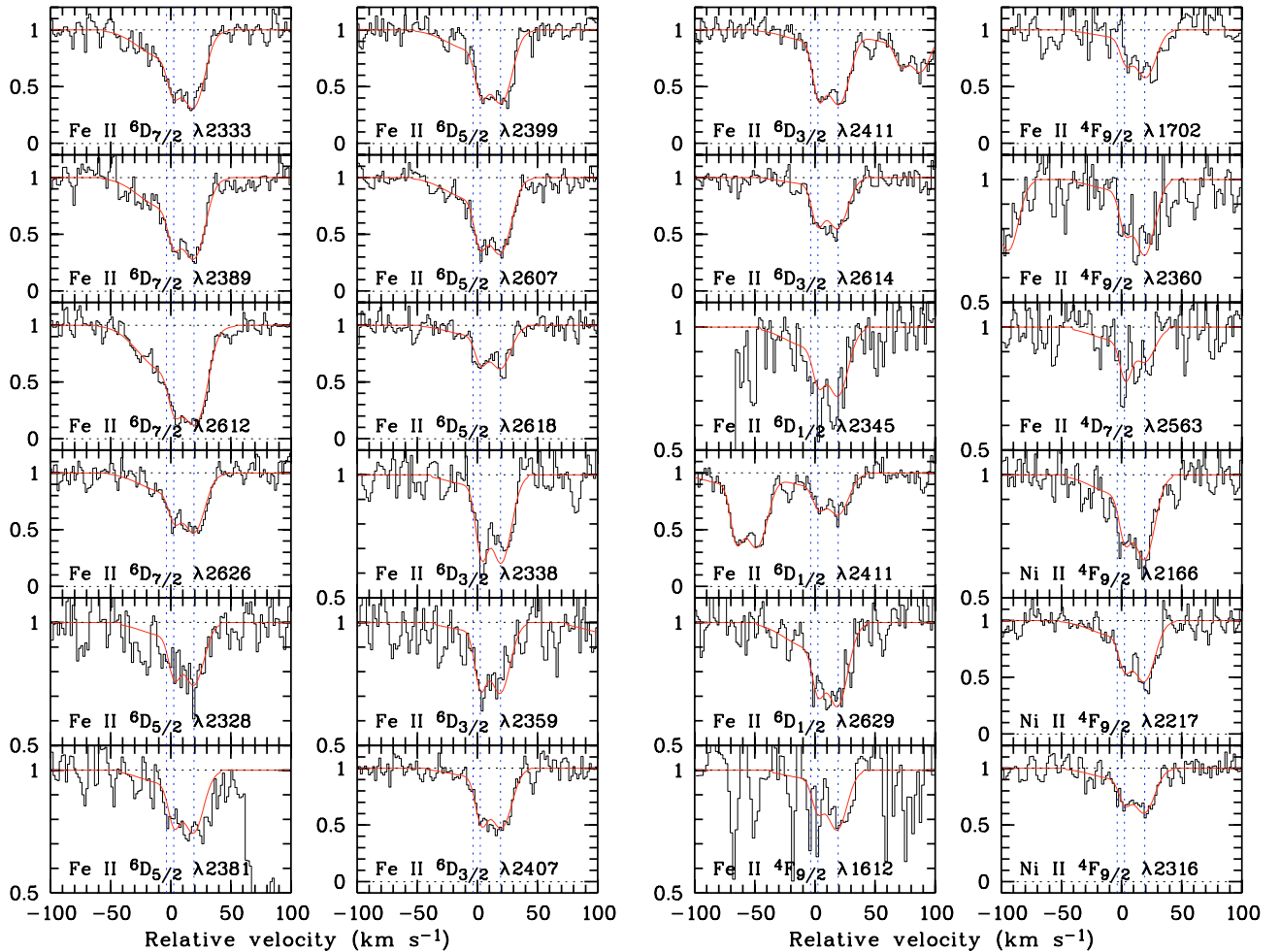
Fig. 3. Absorption-line profile fits to selected transitions from excited Fe II and Ni II. The lower level of the transition, for which the column density is determined from the fits, is indicated in each panel. The fit results are listed in Table 3. We only show the fits for the third epoch spectra; the quality of the spectral fits for the other epochs are very similar, with only small differences due to slightly different signal-to-noise ratios (see Table 1).
