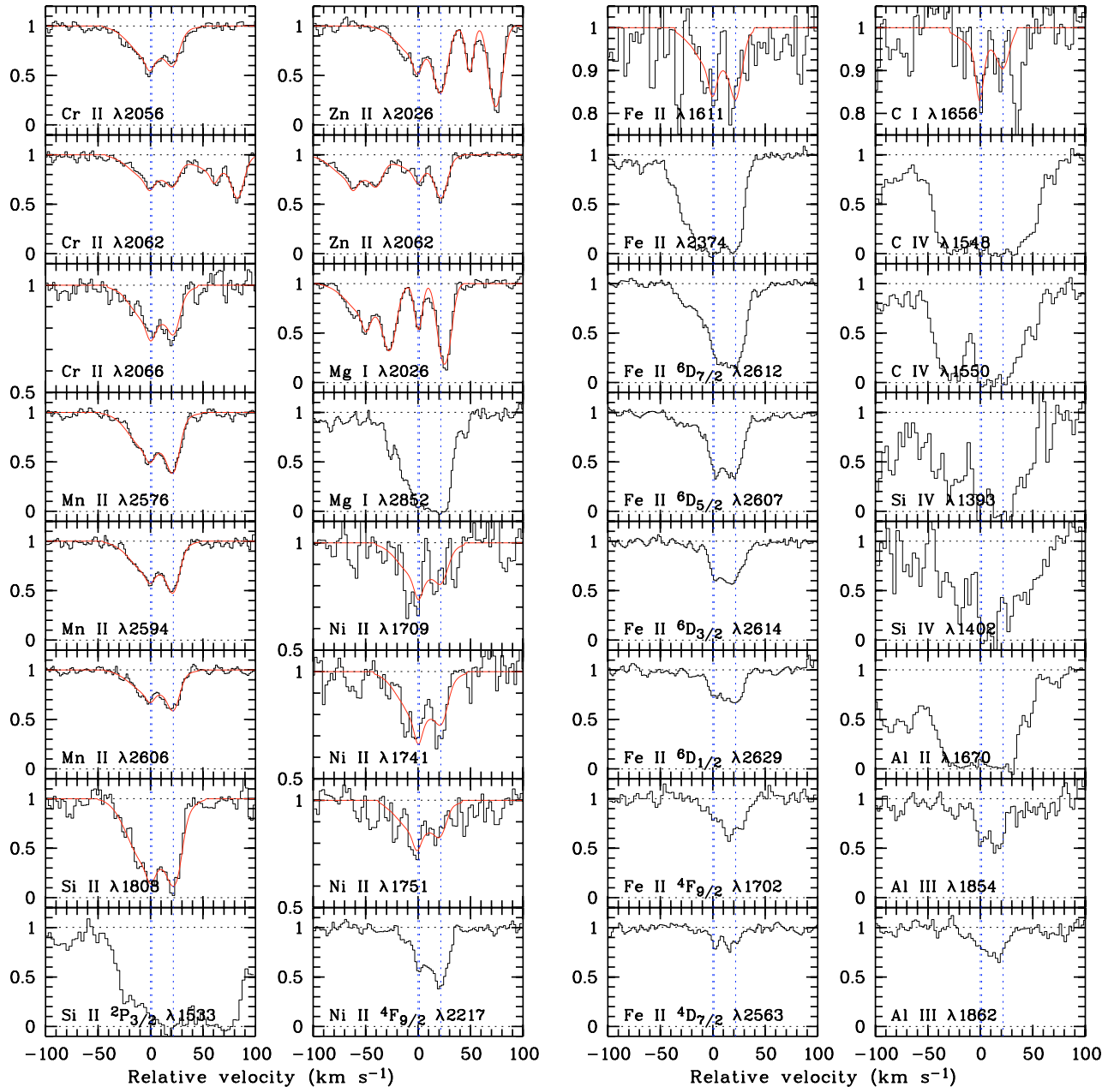
Fig. 1. Absorption-line profiles for a variety of transitions detected at the GRB 060418 redshift. To all low-ionization species containing at least one non-saturated transition, we have performed simultaneous Voigt-profiles fits using a three-component model; the resulting fits are shown by the solid (red) line (see Table 2 for the fit results). The relative velocity of the different components are indicated by the (blue) vertical dotted lines; note that two components have very similar redshifts. It is clear that this 3-component fit does not describe some high S/N lines, such as Zn II \lambda 2026 , very well; we will come back to this in the discussion. We note, however, that the total column density would hardly change if additional components would be introduced. For comparison purposes, we also show transitions that we have not fit: (saturated) higher-ionization lines of C IV and Si IV, lines from Fe II fine-structure levels, and transitions originating from metastable levels of both Fe II and Ni II.
