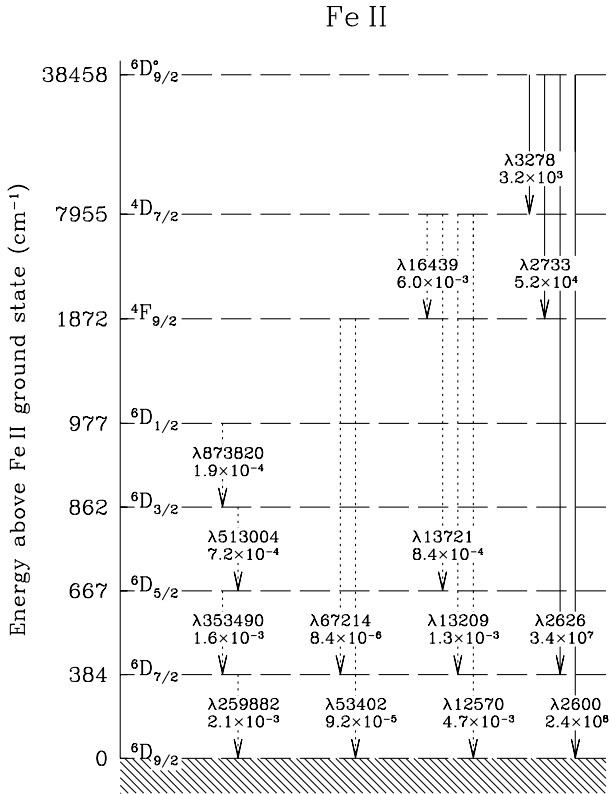
Fig. 4. Energy level diagram for selected levels of Fe II. For the lower levels we only show the levels for which we detect transitions, i.e. the fine-structure levels of the Fe II ground state, and {}^4F_{9/2} and {}^4D_{7/2} . Note that for clarity reasons, we do not show the fine-structure levels of the latter. With the arrows, we indicate the most likely transitions between these levels, including one higher excited level. For each transition we show the wavelength in Å and the spontaneous decay Einstein coefficient, A_{ul} in s^{-1} (which is proportional to the absorption coefficient B_{lu} , see also below). The electric dipole allowed transitions are indicated with a solid line, and the forbidden transitions (magnetic dipole or electric quadrupole) with a dotted line. Note that to populate the level {}^6D_{1/2} , either four IR photons are required, or two UV photons, where the higher levels involved need to have J = 7/2 and J = 3/2 . This, combined with the much larger transition probabilities in the UV, makes the UV pumping mechanism much more efficient than IR excitation.
