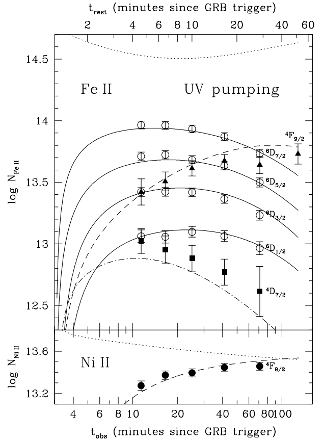
Fig. 8. The top panel shows the same as the top panel of Fig. 6, but now with the UV pumping model overplotted: solid lines for the fine-structure levels, dashed line for {}^4F_{9/2} , and dashed-dotted for {}^4D_{7/2} . The bottom panel displays the observed total column densities for Ni II {}^4F_{9/2} (filled circles), and the best-fit Ni II model. In this Ni II fit, all parameters except for Ni II column density were fixed to the best-fit values obtained from the Fe II fit. The model prediction for the evolution of the Ni II ground state column density is shown by the dotted line. All Fe II and Ni II column densities are very well described by the UV pumping model.
