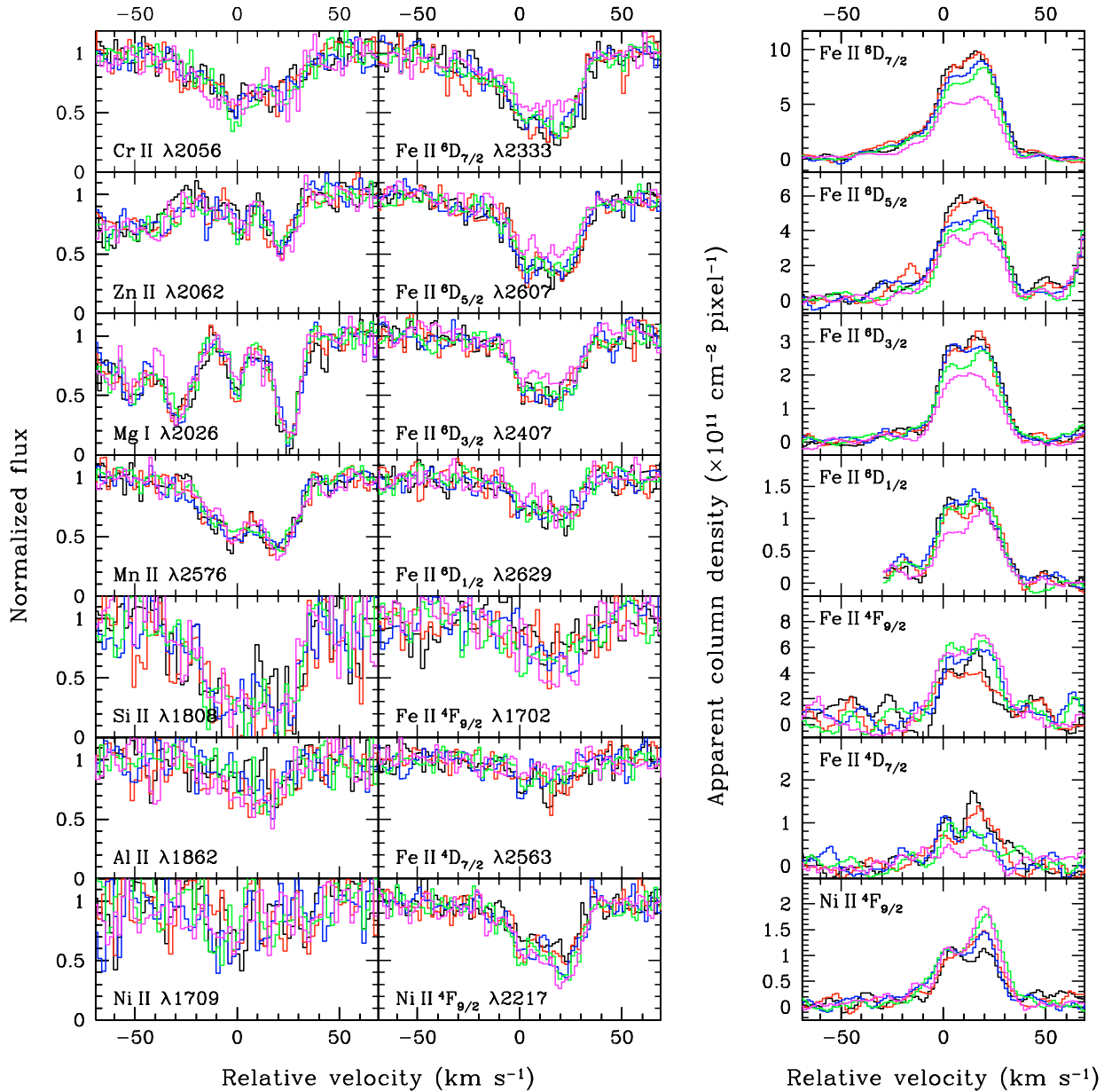
Fig. 2. The epoch 1-5 UVES spectra of GRB 060418 (see Table 1) are overplotted with the colours black, red, blue, green and magenta, respectively. In the left panel individual lines are shown, typical resonance lines on the left, and the lines arising from the excited levels of Fe II and Ni II on the right. The latter show evidence for a varying equivalent width as a function of time. To make this variability clearer, we have combined various lines that arise from the same level and constructed apparent column density profiles, smoothed with a boxcar of 5 pixels; these are shown in the right panel.
