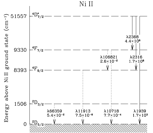
Fig. 5. Energy level diagram for selected levels of Ni II (see Fig. 4). Note the very low A -value for the transition {}^4F_{9/2} to the ground state (this is actually an electric quadrupole transition), while the level {}^4F_{9/2} can be very easily populated from the higher excited levels, one of them being {}^4D_{7/2} . Therefore this level can be expected to be densely populated in the presence of a strong UV radiation field. The fine-structure level of Ni II ground state, {}^2D_{3/2} has a relatively high probability of spontaneous decay, with a mean lifetime of 1/(5.4 \times 10^{-2} \text{ s}^{-1}) = 19 \text{ s} .
