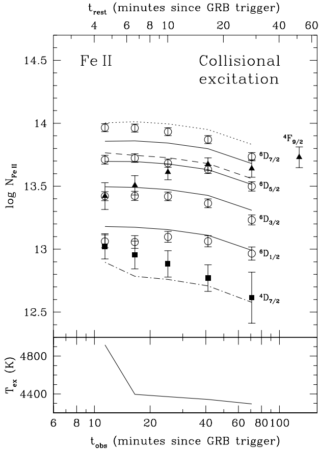
Fig. 6. The top panel shows the observed total column densities (see the last column of Table 3) for the fine-structure lines (open circles; from top to bottom: {}^6D_{7/2} , {}^6D_{5/2} , {}^6D_{3/2} , and {}^6D_{1/2} , respectively), the first metastable level (filled triangles, {}^4F_{9/2} ), and the second metastable level (filled squares, {}^4D_{7/2} ) of Fe II. Overplotted are the results of the best-fit Boltzmann model (collisional scenario): solid lines for the fine-structure levels, dashed line for {}^4F_{9/2} , and dashed-dotted for {}^4D_{7/2} . The best-fit Fe II ground state column density is shown by the dotted line, while the best-fit excitation temperature ( T_{\text{ex}} ) is depicted in the bottom panel. It is clear that the Boltzmann model can be rejected with high confidence.
