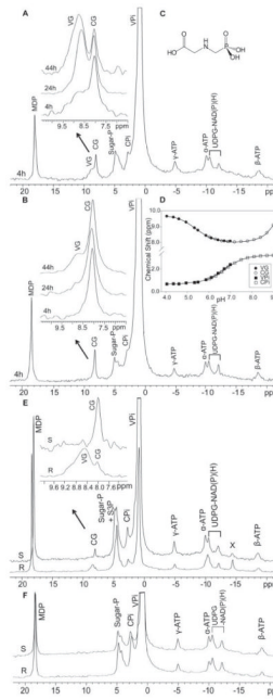
Figure 1. In vivo ^{31}\text{P} NMR spectra of R and S horseweed leaves treated with glyphosate at 3.3 \text{ kg AE ha}^{-1} . A , ^{31}\text{P} NMR spectra of R horseweed source leaves obtained at 4, 24 and 44 h after spraying. B , ^{31}\text{P} NMR spectra of S horseweed source leaves obtained at the same times after spraying. C , Glyphosate chemical structure. D , Glyphosate and Pi ^{31}\text{P} chemical shift dependence as a function of pH determined from standard solutions that mimic environments of the vacuole and cytoplasm: vacuolar glyphosate (●), cytoplasmic glyphosate (○), vacuolar Pi (■), cytoplasmic Pi (□). E , ^{31}\text{P} NMR spectra acquired from R and S horseweed sink leaves 24 h after glyphosate spraying of source leaves. S3P, shikimate-3-phosphate; X indicates an unknown esterified phosphoryl metabolite. F , ^{31}\text{P} NMR spectra of R and S horseweed leaves without glyphosate treatment. Note : 0.00 ppm assigned to 85% phosphoric acid (external) in separate experiments. Abbreviations: MDP, methylene diphosphonate, an external concentration reference; VG, vacuolar glyphosate; CG, cytoplasmic glyphosate; VPi, vacuolar phosphate; CPi, cytoplasmic phosphate; Pi, inorganic phosphate; UDPG, uridine 5'-diphosphoglucose; \alpha -, \beta -, \gamma -ATP refer to corresponding ATP phosphate groups; Sugar-P, sugar phosphates.
