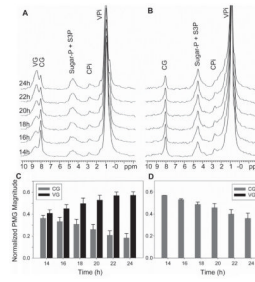
Figure 2. In vivo ^{31}\text{P} NMR time course data for R and S horseweed source leaves collected during the chase phase after a 10 h pulse period with 10 mM glyphosate. A , ^{31}\text{P} NMR stacked plot of data obtained during the chase phase with R horseweed mature leaves. B , ^{31}\text{P} NMR stacked plot of data obtained during the chase phase with S horseweed mature leaves. Each plot represents a 2 h data collection. Note that, at all time periods, glyphosate occupies the cell vacuole (broad signal at 8.68 \pm 0.10 ppm) appreciably in R tissue, whereas little or none is observed in S tissue. C , Total observable glyphosate (PMG, phosphonomethylglycine) during the ‘chase’ period for R horseweed plant tissue ( n = 3 ). For R tissue, glyphosate progressively leaves the cytoplasm (gray) and occupies the vacuole (black) during this period. The Y-axis units are normalized to the external reference MDP signal magnitude. D , Total observable glyphosate during the ‘chase’ period for S horseweed plant tissue ( n = 3 ). Error bars indicate SEM.
