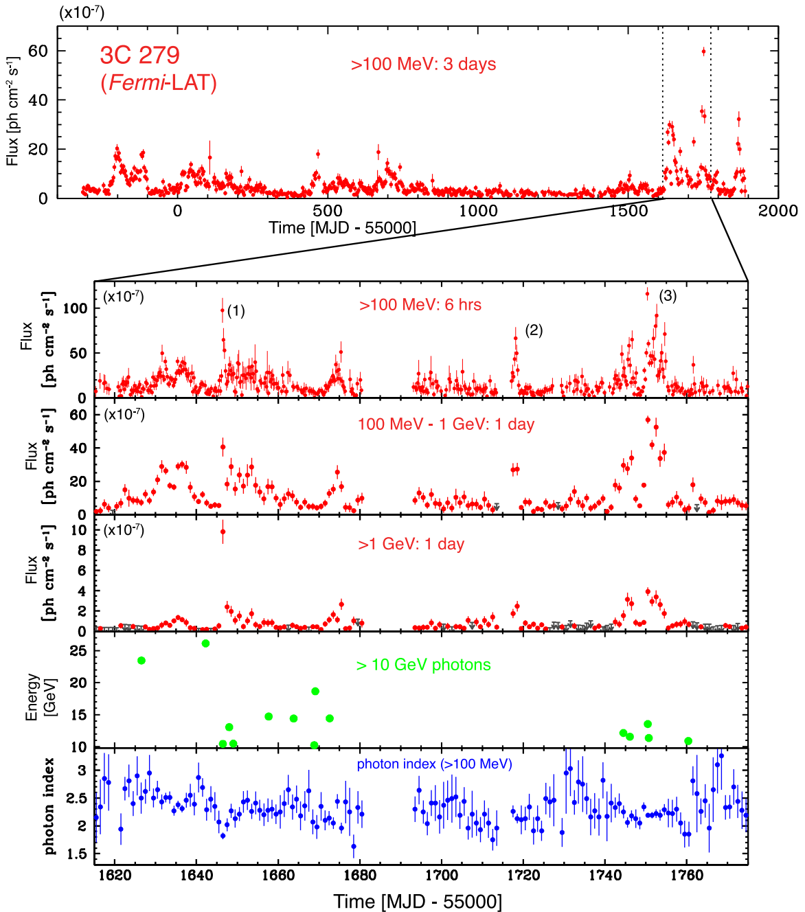
Figure 1. Light curves of 3C 279 in the \gamma -ray band (integral photon flux) as observed by Fermi -LAT. Top panel shows the long-term light curve above 100 MeV in 3 day bins. The other panels show light curves for the 2013–2014 active period: from the top to bottom, (1) above 100 MeV in 6 hr bins, (2) from 100 MeV to 1 GeV in 1 day bins, (3) above 1 GeV in 1 day bins, (4) arrival time distribution of photons with energies above 10 GeV, and (5) photon index of 3C 279 above 100 MeV in 1 day bins. A gap in the data around \sim MJD 56680–56690 is due to a ToO observation of the Crab Nebula, during which time no exposure was available in the direction of 3C 279. The vertical bars in data points represent 1\sigma statistical errors and the down arrows indicate 95% confidence level upper limits.
