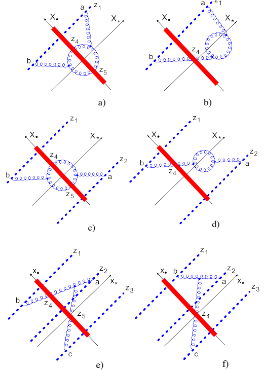
FIG. 2: Typical NLO diagrams.
