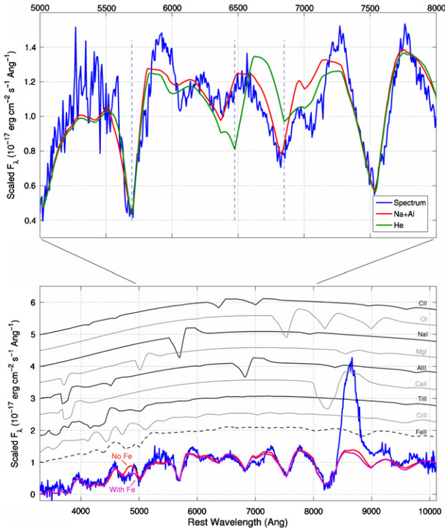
Figure 3. SYNOW fit to the Keck spectrum (+23 days) of SN 2010X. Lines contributed by each ion are shown. Fits with (purple) and without (red) iron are overlotted on the data (blue). Top panel: the dilemma of whether SN 2010X has helium or a combination of sodium and aluminum. The vertical dashed lines show helium at 9500 km s -1 . In non-LTE, the singlet transition of \lambda 6678 may be suppressed relative to the \lambda 7065 and \lambda 5876 triplet transition helium lines. (A color version of this figure is available in the online journal.)
