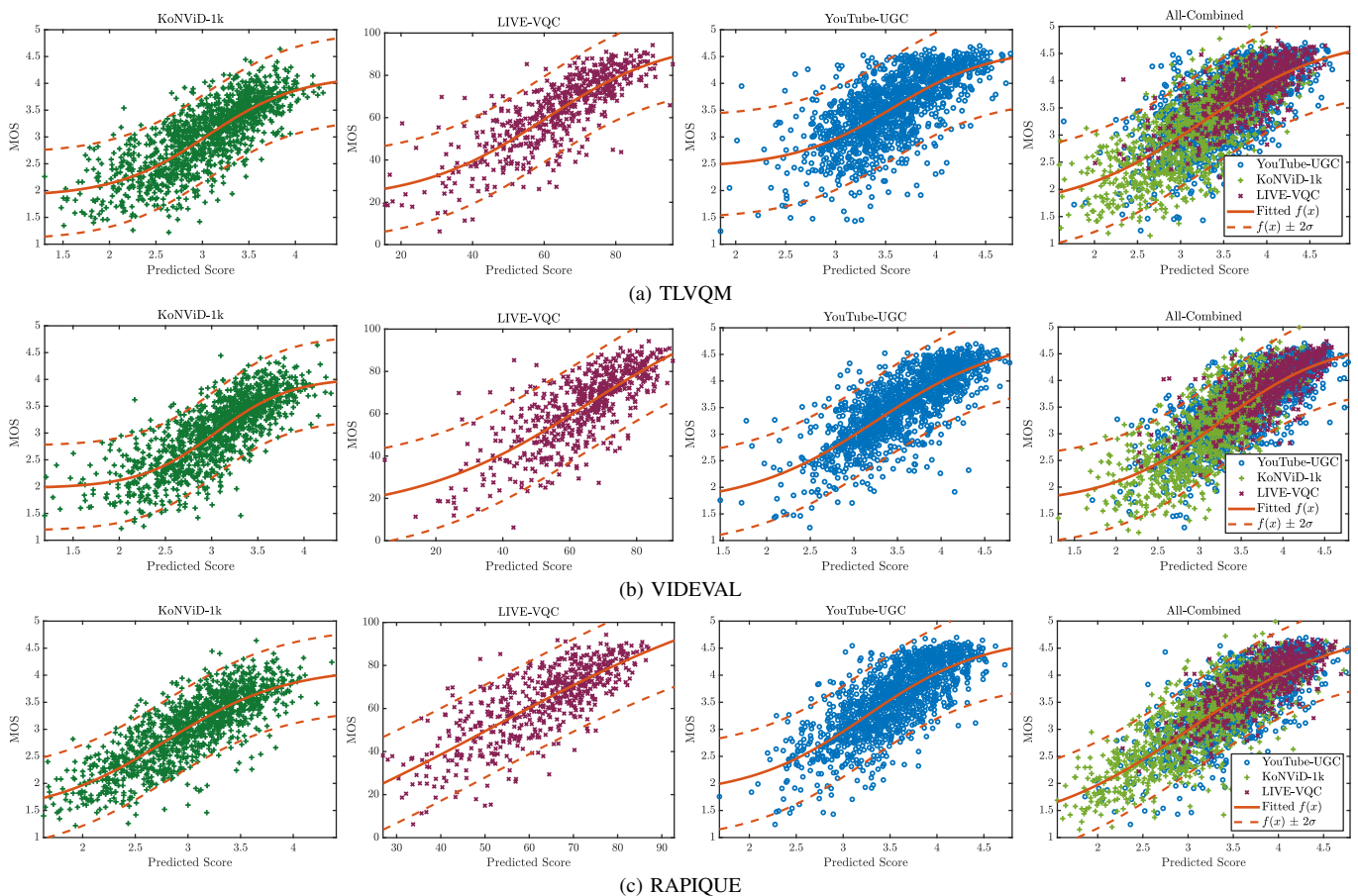
Fig. 9. Scatter plots and nonlinear logistic fitted curves of (c) RAPIQUE versus MOS, compared against (a) TLVQM [13] and (b) VIDEVAL [6], using a grid-search SVR using k -fold cross-validation on KoNViD-1k [31], LIVE-VQC [30], YouTube-UGC [32], and the All-Combined set (Sec. IV-A), respectively.
