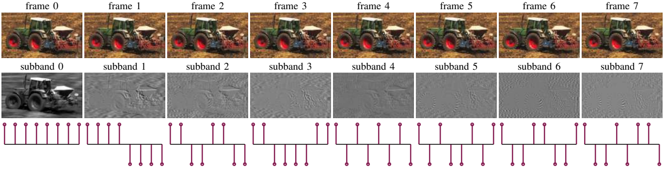
Fig. 7. Top row: eight exemplar consecutive frames sampled from sequence Tractor in LIVE-VQA [1]. Middle row: temporal bandpass-filtered responses by convolving with the filters in an 8-subband Haar-wavelet filter bank, which are shown in the bottom row. The subband frequency increases from left to right: k = 0, \dots, 7 , for both the responses and wavelet functions.
