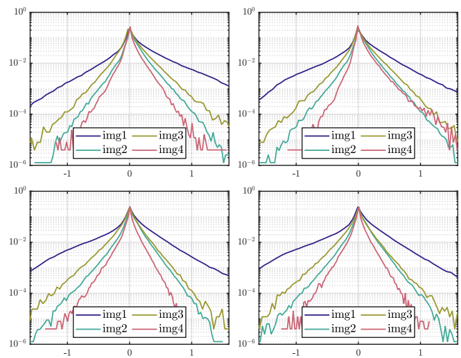
Fig. 4. Histograms of four-orientation (H, V, D1, D2) MSCN pair-production of the four images shown in Fig. 2.
