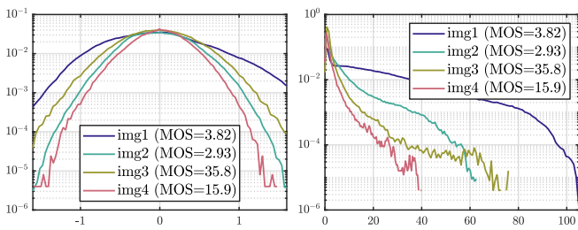
Fig. 3. Histograms of MSCN (left) and variance map (right) of the four images shown in Fig. 2.
