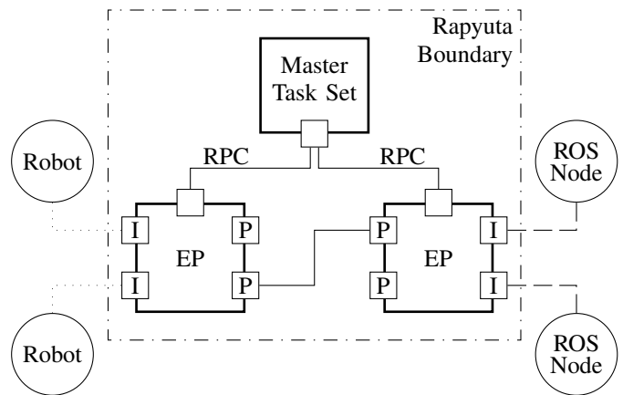
Fig. 2: The basic communication channels of Rapyuta: The Endpoints (EP) are connected to the Master task set using a two-way remote procedure call (RPC) protocol. Additionally, the Endpoints have Interfaces (I) for connections to robots or (ROS) nodes, as well as Ports (P) for communicating between Endpoints . The dotted lines represent the external communication, dashed lines represent the ROS-based communication between ROS nodes and Rapyuta, and finally all solid lines represent the internal communication between Rapyuta's processes.
