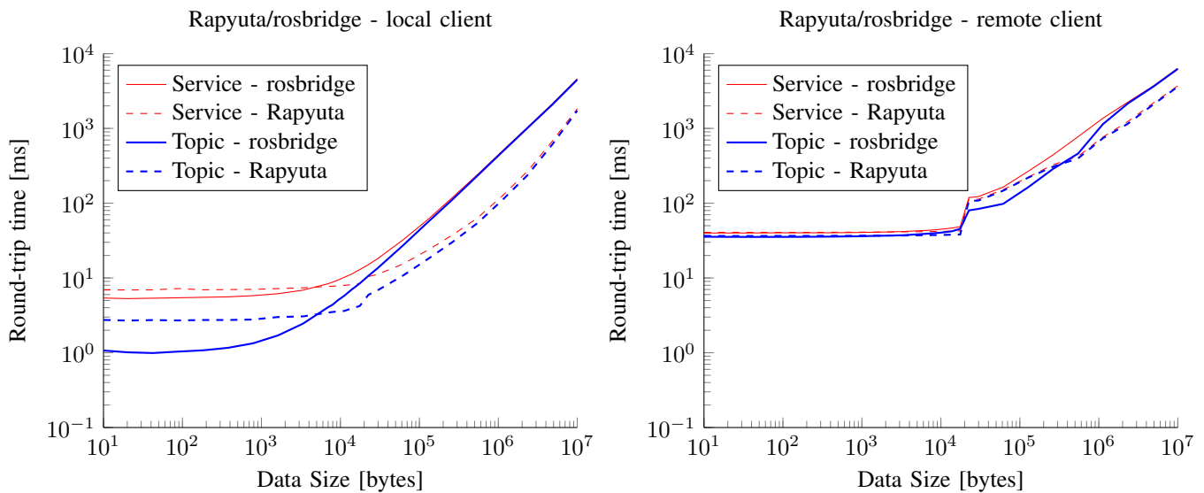
(a) RTTs with the external process running on the same host machine that is running Rapyuta/rosbridge. (b) RTTs with a remote external process running at ETH Zurich, Switzerland while Rapyuta and rosbridge ran on Amazon’s Ireland data center.
