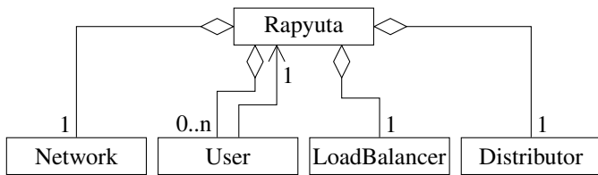
Fig. 3: Simplified UML diagram of Rapyuta's top level command data structure.
