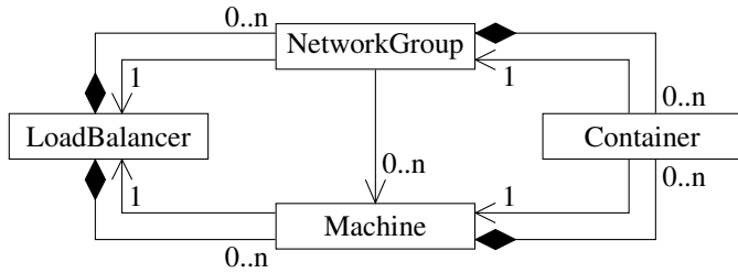
Fig. 6: Simplified UML diagram of Rapyuta's top level component LoadBalancer .
