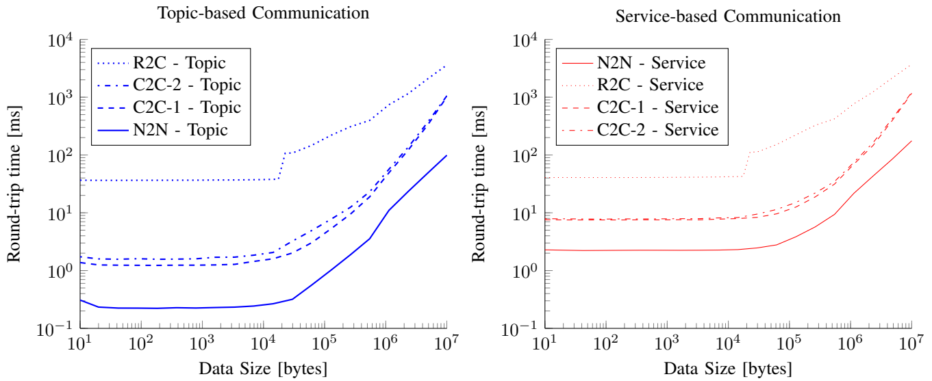
(a) RTTs for different data routes in the standard use case (see Fig. 7) under the topic transport mechanism. (b) RTTs for different data routes in a standard use case (see Fig. 7) under the service transport mechanism.
