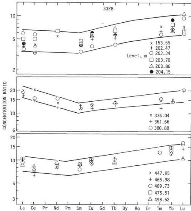
Figure 1b. Rare earth abundance enrichments relative to chondrites as a function of their atomic number.
