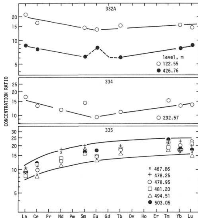
Figure 1a. Rare earth abundance enrichments relative to chondrites as a function of their atomic number.
