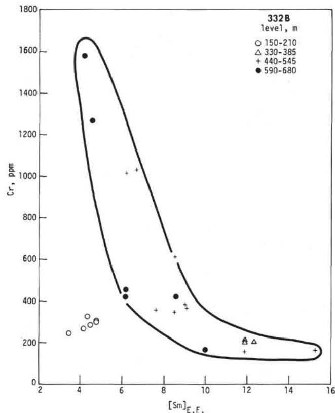
Figure 3. Variation of Cr content versus Sm enrichment factor relative to chondrites for Hole 332B lavas analyzed in this study. Note the inverse relationship between Cr and Sm, except for plagioclase feldspar phyric basalt between the 150-204 meter depth of the drilled core. The highest Cr content are found in Mg-rich-spinel-bearing picrites.
