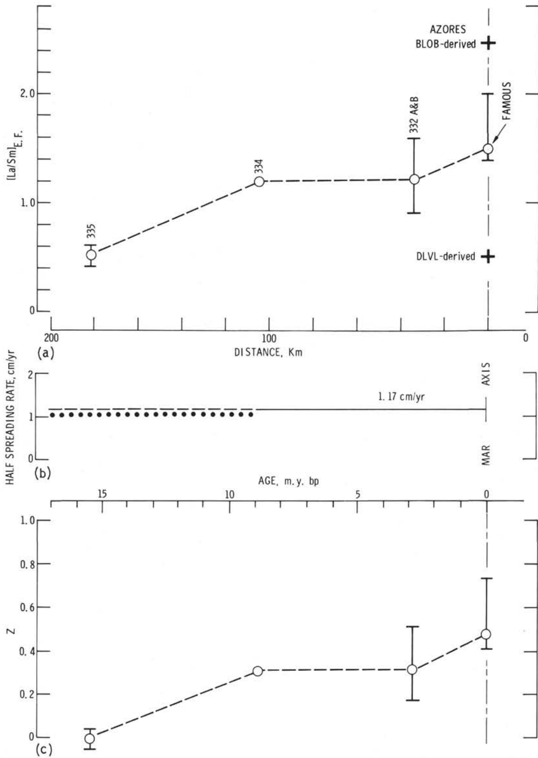
Figure 4. Secular variation of: (a) La/Sm ratio normalized to chondrites; error bars are for maximum variations observed for Holes 332A and 332B and Sites 335, and dredged basalts from FAMOUS area (Schilling, 1975a). (b) Half spreading rates; solid-dashed line from Leg 37 data (this report); dotted line from Pitman and Talwani (1972). (c) Relative mass proportions Z of Azores Mantle Blob component to binary mantle mixture from which lava of Sites 332A, and 334, and 335, and dredged basalts from FAMOUS area are derived. The other mantle source end member component is the low-velocity layer depleted in light RE and large ionic lithophile elements (DLVL). Pure end-member mantle components for present MAR axis are marked by heavy crosses. See also text and Schilling (1973a, 1974, 1975a, b) for explanation of the model.
