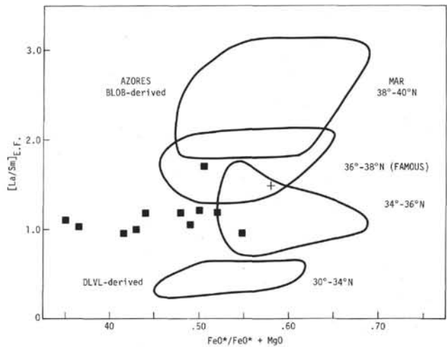
Figure 2. Variation of FeO^*/FeO^*+MgO wt % ratio against chondrite-normalized La/Sm ratio in some basalts from Holes 332B and 332A. Major element data are taken mostly from Sigurdsson (this volume) and three standard rock analyses shown in Wright (this volume). Also shown for comparison are latitudinal variations along the present MAR axis from dredged pillow basalts (Schilling, 1975a). Interpretation of this diagram in terms of partial melting, fractional crystallization, and mantle mixing is given in Schilling (1975a). FeO^* stands for total iron expressed as FeO wt %.
