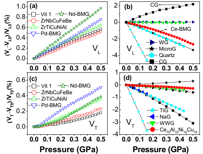
Fig. 17. Pressure dependences of V_L and V_T for \text{Zr}_{41}\text{Ti}_{14}\text{Cu}_{12.5}\text{Ni}_{10.2}\text{Be}_{22.5} (Vit1), \text{Ce}_{70}\text{Al}_{10}\text{Ni}_{10}\text{Cu}_{10} , \text{Zr}_{48}\text{Nb}_8\text{Cu}_{12}\text{Fe}_8\text{Be}_{24} , \text{Zr}_{50.6}\text{Ti}_{5.2}\text{Cu}_{18.8}\text{Ni}_{14.1}\text{Al}_{14.3} , \text{Nd}_{60}\text{Al}_{10}\text{Fe}_{20}\text{Co}_{10} , \text{Pd}_{39}\text{Ni}_{10}\text{Cu}_{30}\text{P}_{21} , amorphous carbon (CG) and oxide glasses. The oxide glasses are window glass (WG), water white glass (WWG), fused quartz (Quartz), floats glass (NaG) and \text{SiO}_2 + \text{TiO}_2 glass (TiG).
