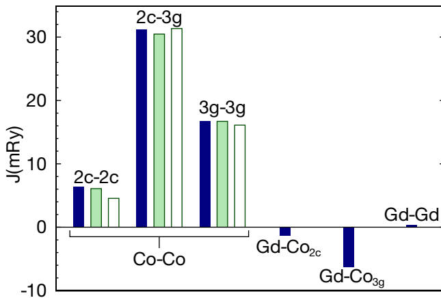
FIG. 5. Calculated values of J_{ij} in the high-temperature expansion of equation 7 for GdCo 5 (blue) and YCo 5 (green). The empty bars are the values of J_{ij} computed for YCo 5 using the lattice parameters of GdCo 5 (see text).
