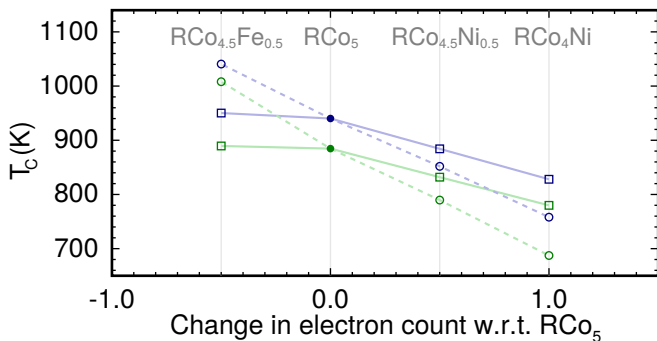
FIG. 10. Curie temperatures calculated for \text{YCo}_5 (green) and \text{GdCo}_5 (blue) for different doping concentrations, where the dopants have been substituted either at \text{Co}_{2c} (circles, dashed lines) or \text{Co}_{3g} (squares, solid lines) sites.
