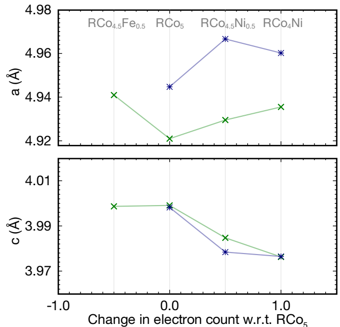
FIG. 13. Lattice parameters (in Å) measured by powder x-ray diffraction for the as-cast samples of transition metal-doped \text{YCo}_5 (green, crosses) and \text{GdCo}_5 (blue, stars).
