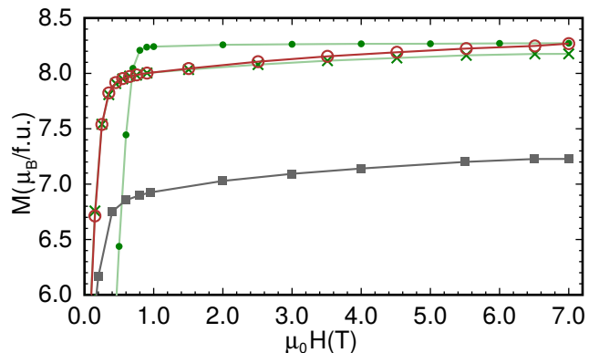
FIG. 9. Magnetization vs. applied field measured at 5 K for single crystal \text{YCo}_5 (green line, filled circles), polycrystalline (powdered) \text{YCo}_5 (green line, crosses), \text{YCo}_{4.5}\text{Ni}_{0.5} (gray line, squares) and \text{YCo}_{4.5}\text{Fe}_{0.5} (brown line, empty circles).
