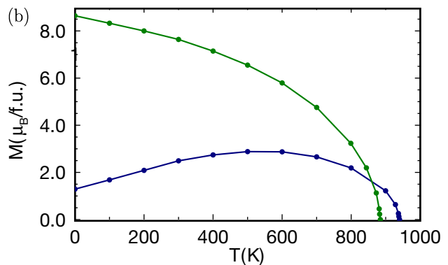
FIG. 2. Magnetization vs temperature (a) measured on single-crystal samples and (b) calculated in the DLM picture, for \text{YCo}_5 (green) and \text{GdCo}_5 (blue). The straight lines connecting points in (b) are guides to the eye.
