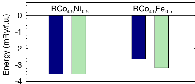
FIG. 7. Calculated energetics of doping of \text{GdCo}_5 (blue) or \text{YCo}_5 (green) by substituting at a \text{Co}_{2c} site. The y -axis zero corresponds to the energy per formula unit when the dopant is substituted at a \text{Co}_{3g} site, i.e. negative bars imply the dopant is more stable sitting at a \text{Co}_{2c} site.
