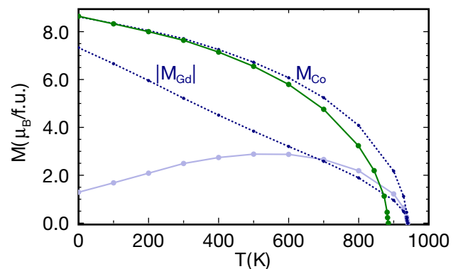
FIG. 4. Decomposition of the magnetization of \text{GdCo}_5 (faint solid blue line) into contributions from the Gd and Co sublattices M_{\text{Gd}} and M_{\text{Co}} (dotted lines, small circles). Note that the sublattice magnetizations point antiparallel, so the resultant magnetization is M_{\text{Co}} - |M_{\text{Gd}}| . The calculated magnetization of \text{YCo}_5 (green solid line) is also shown for comparison.
