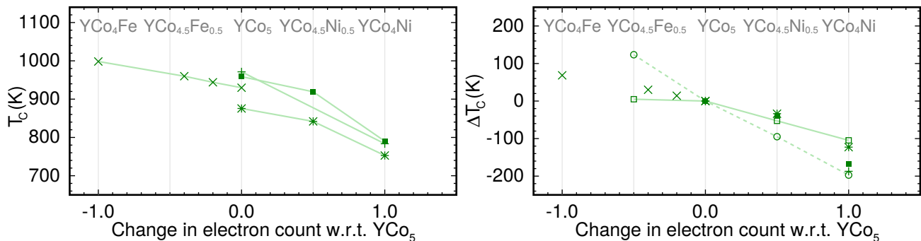
FIG. 11. Curie temperatures of doped YCo_5 , shown on an absolute scale (left panel) or relative to the T_C measured/calculated for pristine YCo_5 (right panel). The experimental T_C values were previously reported in Refs. 40 (diagonal crosses), 33 (filled squares), 35 (upright crosses) and 32 (asterisks). The right panel additionally shows the calculated T_C values for doped YCo_5 (cf. Fig. 10) with the dopants at Co_{2c} (circles, dashed lines) or Co_{3g} (empty squares, solid lines) sites.
