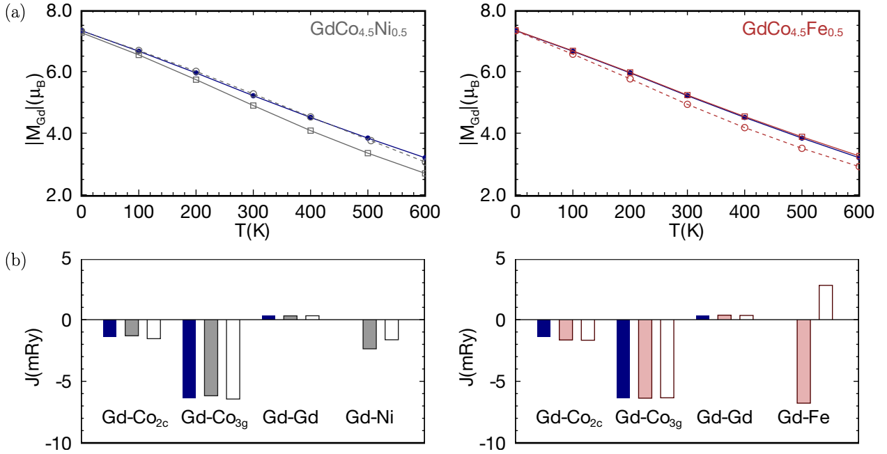
FIG. 12. (a) Absolute magnetization of the Gd sublattice and (b) calculated J parameters for Ni or Fe-doped \text{GdCo}_{4.5}\text{T}_{0.5} . Doping on the \text{Co}_{2c} or \text{Co}_{3g} site is denoted in (a) by empty circles and squares, respectively, and by empty and light-filled bars in (b). Dark blue filled circles/bars correspond to pristine \text{GdCo}_5 .
