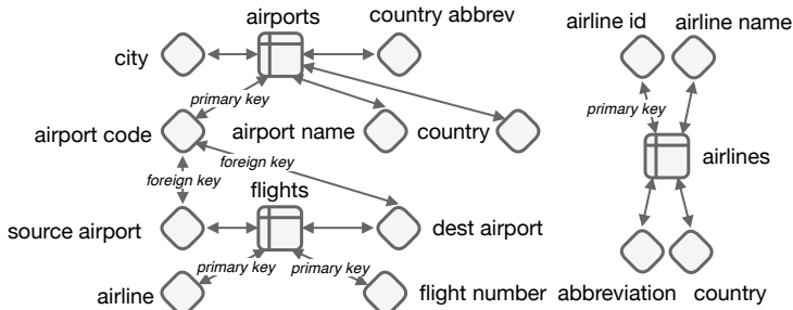
Figure 2: An illustration of an example schema as a graph. We do not depict all edges and label types of Table 1 to reduce clutter.
