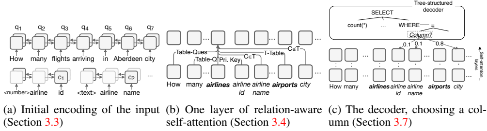
Figure 3: Overview of the stages of our approach.
