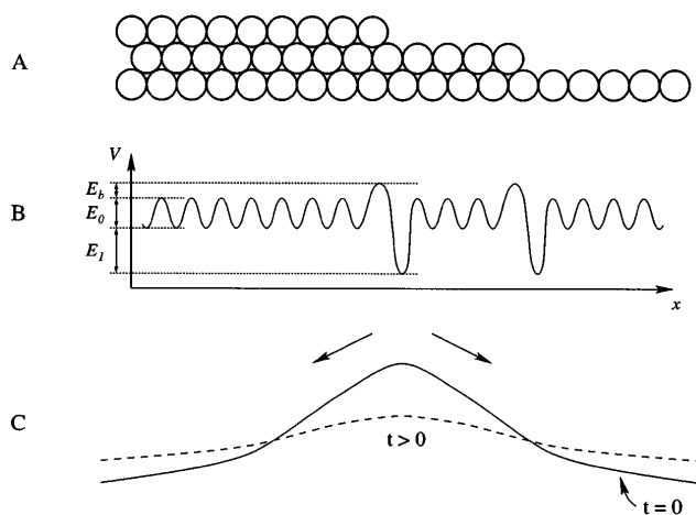
FIG. 1. Schematic illustration of the cross section of a vicinal surface containing two monatomic steps (A) and the asymmetric lattice potential (B) experienced by an atom diffusing on this surface. Note that if the Schwoebel barrier E_b = 0 , the lattice potential near a step is spatially symmetric, while this symmetry is broken for E_b \neq 0 . A downhill (uphill) current points to the right (left) on this figure. As (C) illustrates, if there is a mound on the surface at t = 0 , a downhill current indicated by the arrows will tend to decrease its height; i.e., it smoothes the film by the reorganization of the material on the surface.
