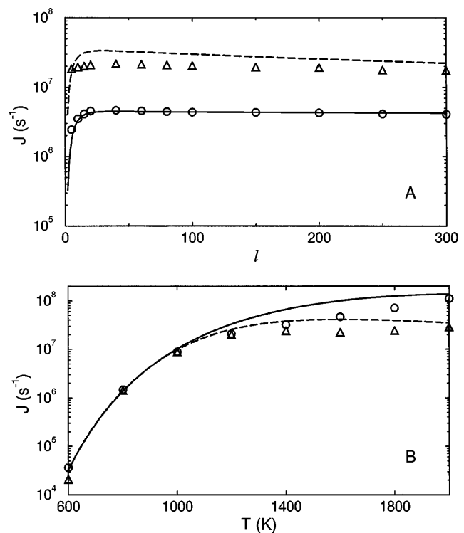
FIG. 3. (A) The ac field induced downhill current as a function of the average step size \ell . The lines correspond to the analytical results (2) and (3) for T = 900 K (continuous line) and T = 1200 K (dashed line), while the circles (900 K) and triangles (1200 K) are the currents predicted by the MC simulations. (B) The temperature dependence of the net current for average step sizes \ell = 20 and \ell = 200 . The continuous ( \ell = 20 ) and dashed ( \ell = 200 ) lines correspond to the analytical predictions, while the circles ( \ell = 20 ) and triangles ( \ell = 200 ) are the result of the MC simulations. In the simulations we used the parameters E_0 = 0.3 eV, E_1 = 0.6 eV, E_b = 0.15 eV, Z = 0.5 , E = 10^8 V/m, and \nu_0 = 10^{13} s -1 . The system size is L = 2000 , and the results were averaged over 20 independent runs.
