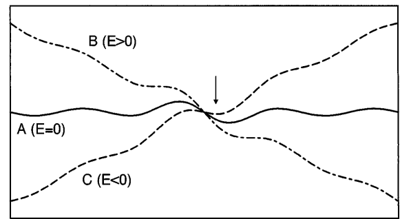
FIG. 2. The effect of a uniform electric field on the potential landscape experienced by an atom diffusing on the surface. The line A corresponds to the lattice potential in the vicinity of a step for E = 0 [see also Fig. 1(B)]. Assuming Z > 0 , a large enough field to the right ( E > 0 ) “tilts” the potential landscape, eliminating the minima of the potential, biasing the adatom motion to the right (see B). On the other hand, as C illustrates, an inverse field ( E < 0 ) of the same magnitude does not eliminate the minima in the vicinity of the step (marked by an arrow), locally trapping the particle. Consequently, the current to the left in C is smaller than the current to the right in B, and a periodic external field will result in a net current to the right, i.e., a downhill current. For smaller fields there are minima in both cases, but the minimum corresponding to C is deeper than that of B, again resulting in a more efficient trapping of the atoms moving uphill, and to a net downhill current. Note that the direction of the net current is determined only by the step orientation, and not by the sign of Z .
