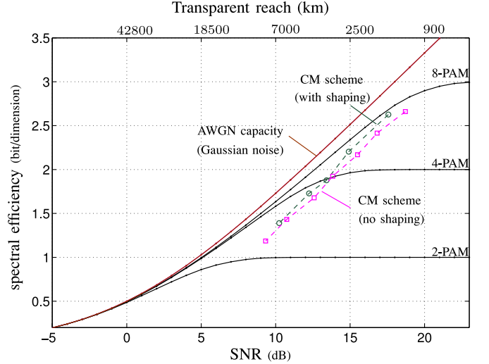
Fig. 8. The spectral efficiency per dimension versus the transparent reach and the SNR for a non-DM link with EDC. The CM scheme curves are based on the results given in Tables V and IV and the spectral efficiency for the Gaussian noise model is computed by (1/2) \log_2(1 + \text{SNR}) , where \text{SNR} = |\zeta|^2 P / \sigma_{z_x}^2 .
