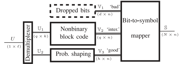
Fig. 6. The encoder for the proposed CM scheme, consisting of a block code, a 4D mapper, and a probabilistic shaping unit.
