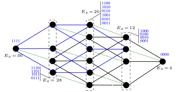
Fig. 5. The labeling bits v_5 v_6 v_7 v_8 of ‘good’ subchannels shown in Table II(b) for the first subset \mathcal{A}_0 \times \mathcal{A}_0 \times \mathcal{A}_0 \times \mathcal{A}_0 of PM 16-QAM. This labeling is suitable for probabilistic signal shaping.
