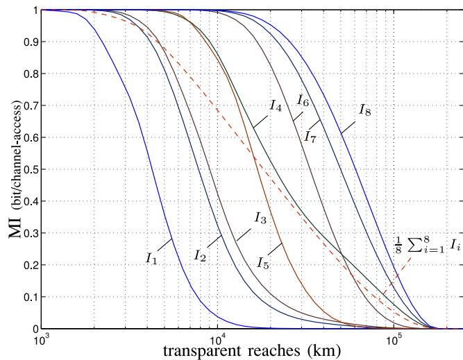
Fig. 4. The bitwise conditional MIs for a 4D mapper with PM 16-QAM. The fiber-optic link is implemented with the parameters given in Table I.
