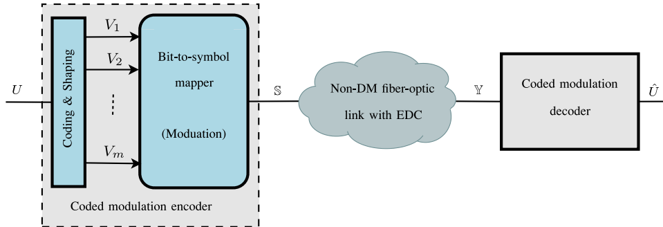
Fig. 1. A non-DM fiber link including a CM encoder at the transmitter, a non-DM fiber-optic channel with N spans, each consisting of an SMF and an EDFA, and the CM decoder and EDC at the receiver ( U is the input information bit sequence and \hat{U} is the decoded bit sequence).
