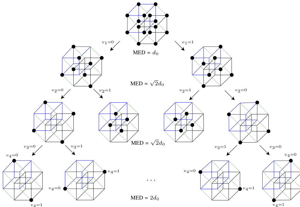
Fig. 3. First four steps of the 4D set partitioning of PM 16-QAM. Black circles represent the subsets given in Table II(a). The first four bits of the binary labeling for this constellation are represented by v_4 v_3 v_2 v_1 .
