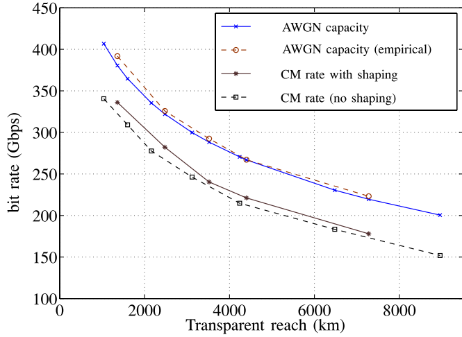
Fig. 7. Bit rates per two polarizations achieved by the CM scheme versus the transparent reach of a non-DM link with EDC, with and without probabilistic shaping.
