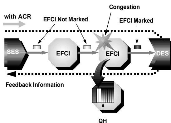
Figure 1: Basic Configuration of the Rate-Based Congestion Control.
