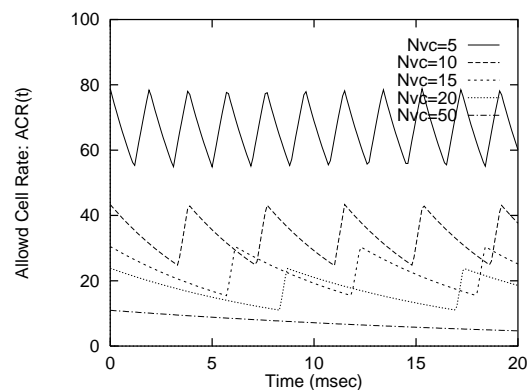
Figure 8: Effect of N_{VC} on ACR(t) in an EFCI Switch ( \tau = 0.02 msec).
