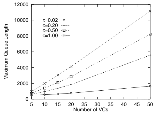
Figure 12: Effect of N_{VC} on the Maximum Queue Length in an EFCI Switch.
