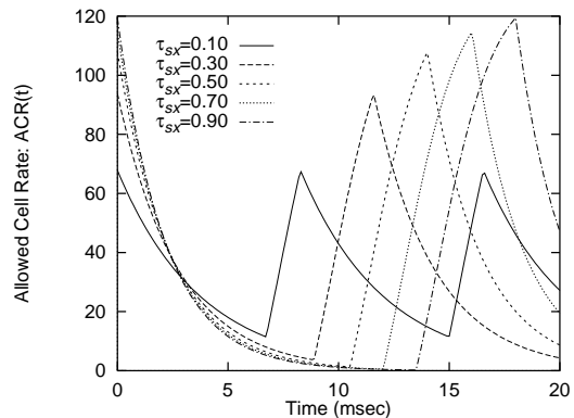
Figure 13: Effect of Switch Location on ACR(t) in a BES Switch ( N_{VC} = 10, \tau_{sx} + \tau_{xd} = 1 ).
