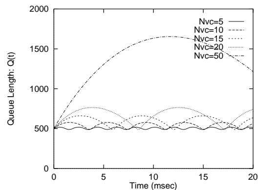
Figure 9: Effect of N_{VC} on Q(t) in an EFCI Switch ( \tau = 0.02 msec).
