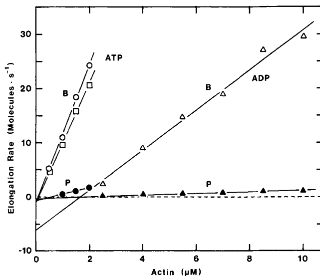
Figure 5. Elongation rates at the barbed (open symbols) and pointed (solid symbols) ends of actin filaments as a function of the concentration of ATP-actin (open and solid circles, open squares) and ADP-actin (open and solid triangles). Conditions: 50 mM KCl, 1 mM MgCl 2 , 1.1 mM EGTA, 0.5 mM DTT, 22°C. As described in detail in Materials and Methods, Mg-ATP-actin (circles) was treated with hexokinase and glucose to convert it to Mg-ADP-actin (triangles) and then at the completion of the experiments with Mg-ADP-actin, it was reconverted to Mg-ATP-actin (open squares) with excess ATP. The pointed end rates with Mg-ATP-actin before and after conversion to Mg-ADP-actin were the same.
