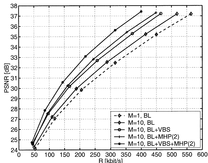
Fig. 11. Average luminance PSNR over total rate for the sequence Mobile & Calendar . Multihypothesis and VBS prediction can be successfully combined for compression. M = 10 reference pictures are utilized for prediction.
