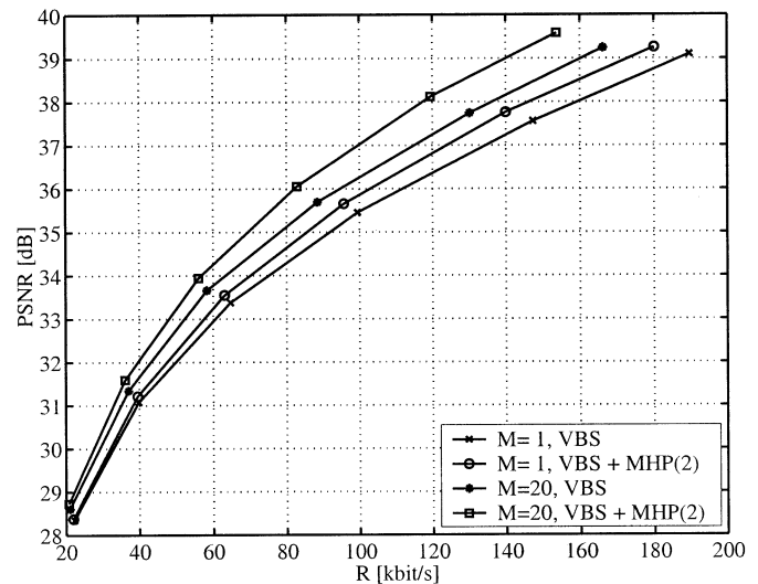
Fig. 14. Average luminance PSNR over total rate for the sequences Foreman . The performance of the multihypothesis codec with VBS is depicted for M = 1 and M = 20 reference frames.
