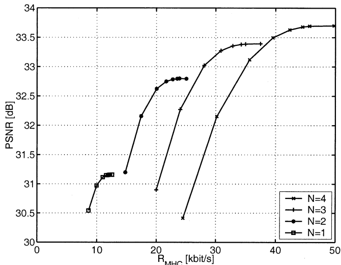
Fig. 3. Quality of the prediction signal versus rate of the N -hypothesis code for the sequence Foreman (QCIF, 10 fps, 10 s), 16 \times 16 blocks, half-pel accuracy, and M = 10 .
