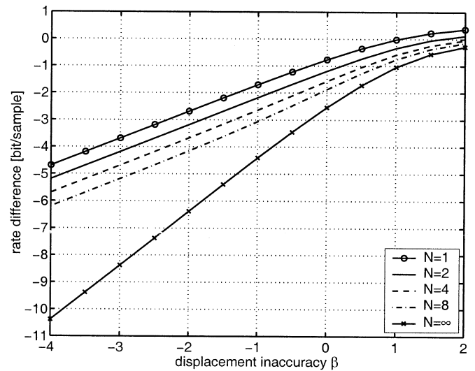
Fig. 6. Rate difference for multihypothesis MCP over the displacement inaccuracy \beta for statistically independent displacement error. The hypotheses are averaged and no residual noise is assumed.
