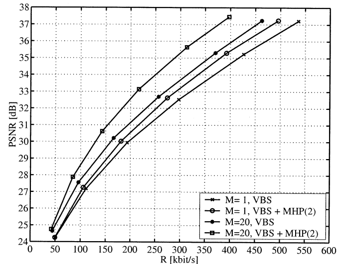
Fig. 15. Average luminance PSNR over total rate for the sequences Mobile & Calendar . The performance of the multihypothesis codec with VBS is depicted for M = 1 and M = 20 reference frames.
