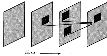
Fig. 1. Multihypothesis MCP with three hypotheses. Three blocks of previous decoded frames are linearly combined to form a prediction signal for the current frame.
