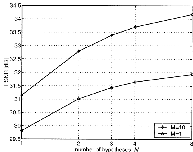
Fig. 2. Quality of the prediction signal and the number of hypotheses N for the sequence Foreman (QCIF, 10 fps, 10 s), 16 \times 16 blocks, half-pel accuracy, and no rate constraint. M indicates the number of reference frames.
