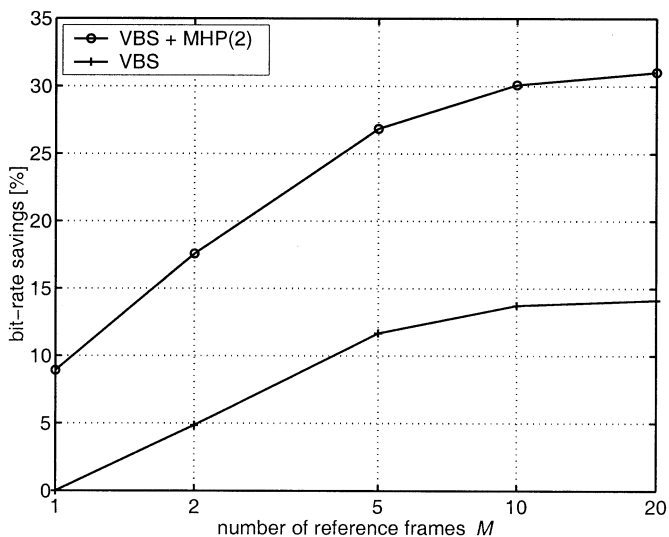
Fig. 13. Bit-rate savings at 35-dB PSNR over number of reference pictures for the sequence Mobile & Calendar . The performance of the multihypothesis codec with VBS is depicted for a variable number of reference frames M .
