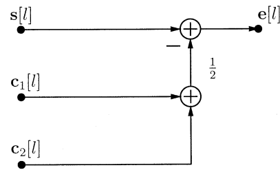
Fig. 4. Multihypothesis MCP with two hypotheses. The current frame s[l] is predicted by averaging two hypotheses c_1[l] and c_2[l] .
