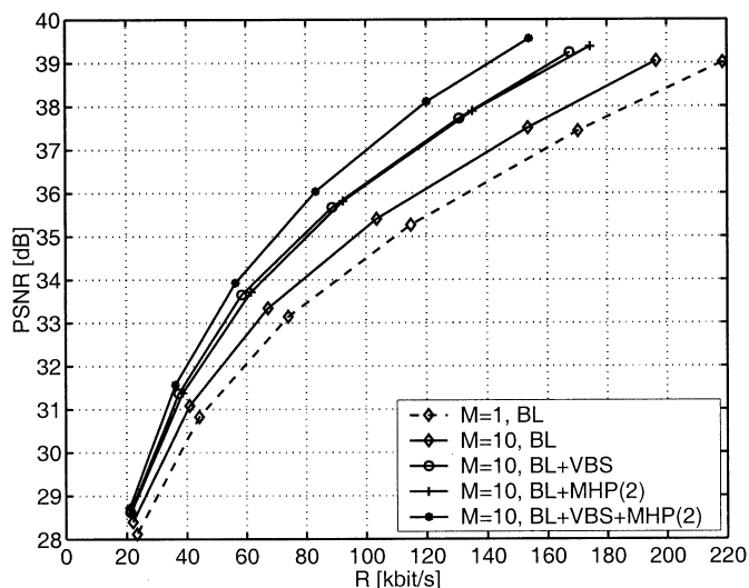
Fig. 10. Average luminance PSNR over total rate for the sequence Foreman . Multihypothesis and VBS prediction can be successfully combined for compression. M = 10 reference pictures are utilized for prediction.
