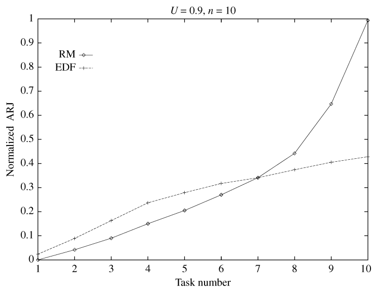
Figure 13. Average normalized jitter for U = 0.9 .
