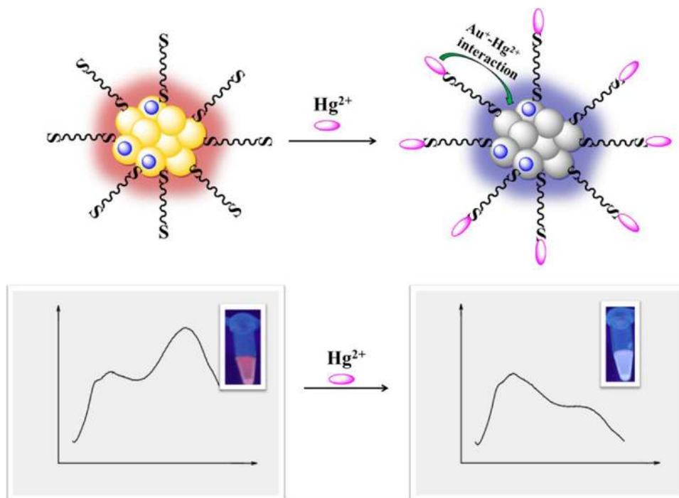
Fig. 4. Schematic illustration of the proposed quenching mechanism of the sensor for \text{Hg}^{2+} detection.
