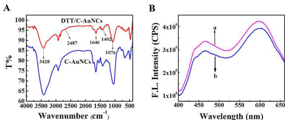
Fig. 3. (A) The FT – IR spectra of C-AuNCs and DTT/C-AuNCs. (B) The fluorescence spectra ( \lambda_{\text{ex}} = 380 \text{ nm} ) of C-AuNCs (a) before and (b) after DTT modification.
