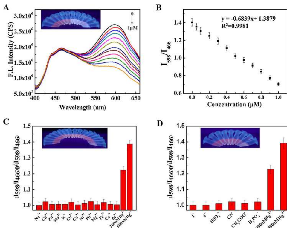
Fig. 5. (A) Fluorescence emission spectra ( \lambda_{\text{ex}} = 380 \text{ nm} ) of 0.20 mg/mL DTT/C–AuNCs in the presence of different concentrations of \text{Hg}^{2+} . Spectra were recorded after 10 min upon addition of \text{Hg}^{2+} in the working solution at room temperature. (B) The linear relationship between the fluorescence ratios ( I_{598}/I_{466} ) and the concentrations of \text{Hg}^{2+} range from 0 to 1 \mu\text{M} . (C) Selectivity of 0.20 mg/mL DTT/C–AuNCs toward \text{Hg}^{2+} together with other cations ( \text{Na}^+ , \text{Cd}^{2+} , \text{Zn}^{2+} , \text{Mn}^{2+} , \text{K}^+ , \text{Co}^{2+} , \text{Cu}^{2+} , \text{Ni}^{2+} , \text{Pb}^{2+} , \text{Mg}^{2+} , \text{Fe}^{3+} , \text{Ca}^{2+} , \text{Ba}^{2+} ) at concentration of 500 nM. (D) Selectivity of 0.20 mg/mL DTT/C–AuNCs toward \text{Hg}^{2+} together with anions ( \text{I}^- , \text{F}^- , \text{HSO}_4^- , \text{CN}^- , \text{CH}_3\text{COO}^- , \text{H}_2\text{PO}_4^- ) at a concentration of 500 nM. The insert photos show the corresponding fluorescence colors change of the working solution under a UV lamp.
