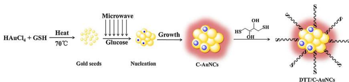
Fig. 1. Schematic illustration of the synthetic routes of DTT/C-AuNCs.
