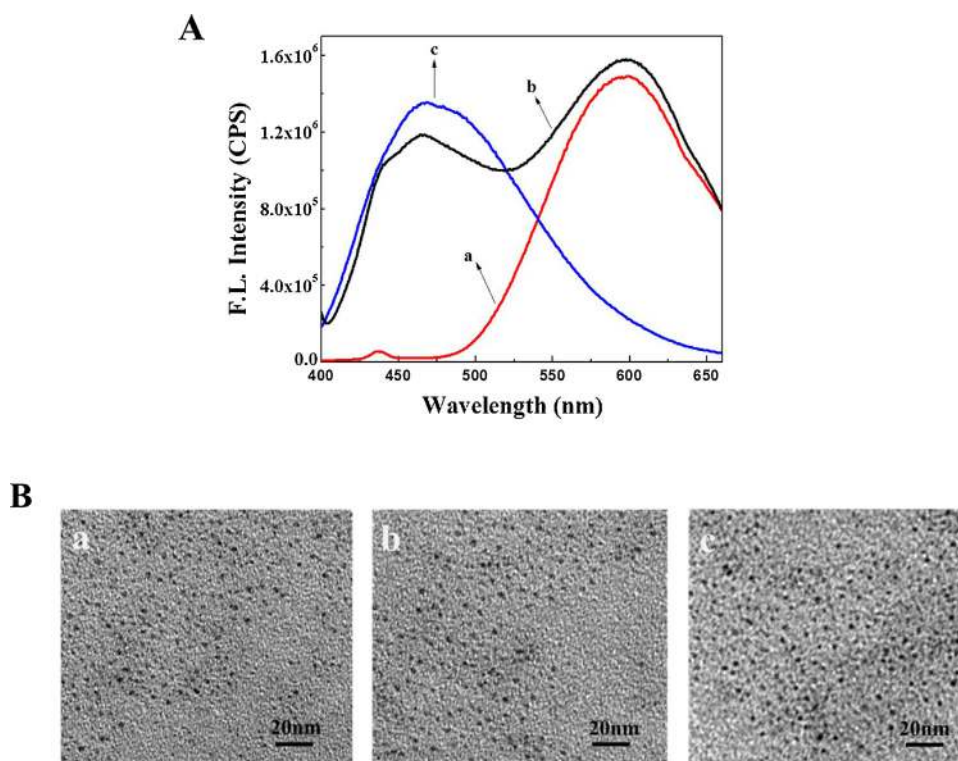
Fig. 2. (A) Fluorescence emission spectra ( \lambda_{\text{ex}} = 380 \text{ nm} ) of (a) AuNCs, (b) C-AuNCs, and (c) DTT/C-AuNCs. (B) TEM images of (a) AuNCs, (b) C-AuNCs and (c) DTT/C-AuNCs.
