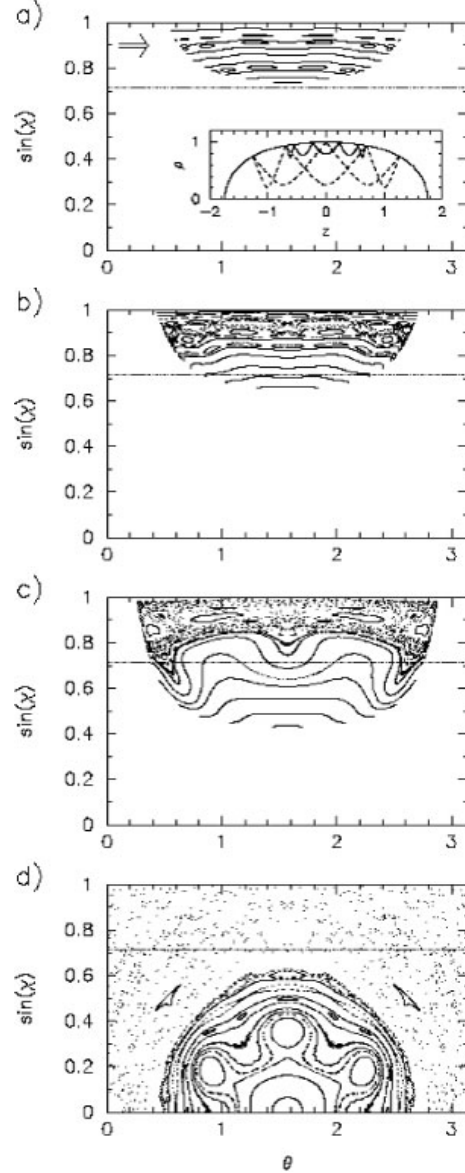
Figure 2: Poincaré surfaces of section for prolate droplets with deformation of \epsilon = 0.3 for L_z = 0.735 (a), L_z = 0.65 (b), L_z = 0.43 (c) and L_z = 0 (d). The arrow to the left indicates the angle of incidence at which the ray bundle is launched, \sin \chi_0 \approx 0.9 , dash-dotted line denotes \sin \chi_c = 1/n = .735 for the droplets of Fig. 1. Inset in (a) shows the droplet shape in the z - \rho plane and typical trajectories for L_z = 0.735 (solid line) and L_z = 0.2 (dashed line).
